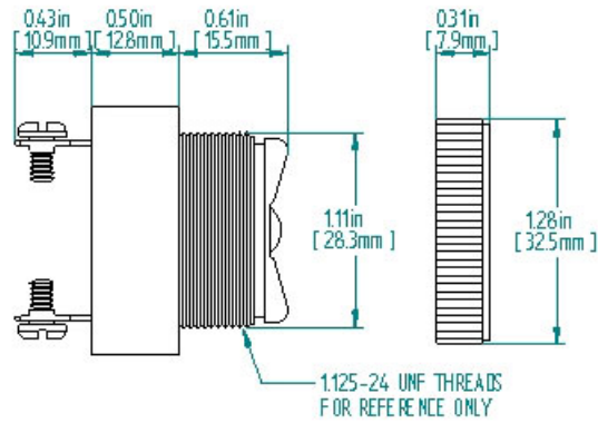
SIDE
