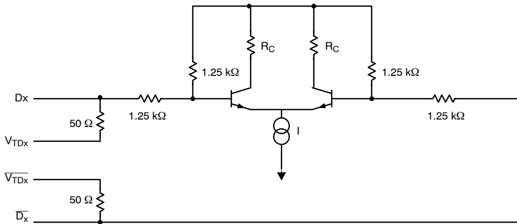
Figure 6. Input Structure
