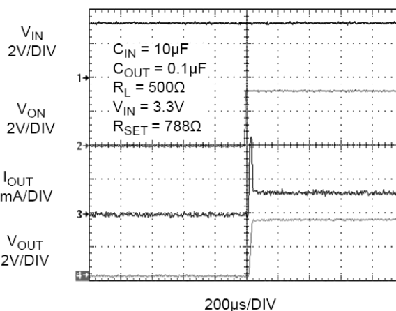
Figure 18. t_{ON} Response
