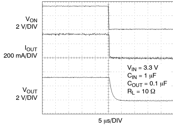
Figure 17. PPF1005 T_{OFF} Response
