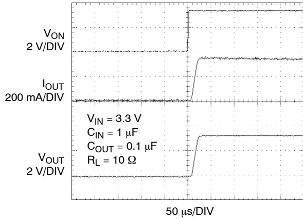
Figure 16. PPF1005 T_{ON} Response
