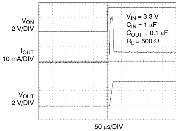
Figure 18. PPF1006 T_{ON} Response
