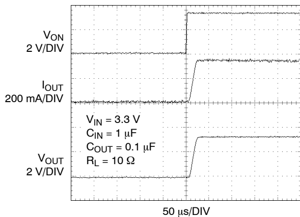
Figure 20. PPF1006 T_{ON} Response
