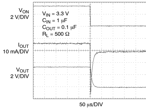
Figure 19. PPF1006 T_{OFF} Response
