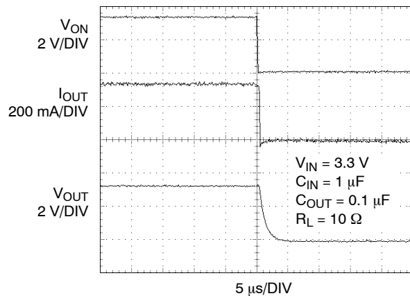
Figure 21. PPF1006 T_{OFF} Response
