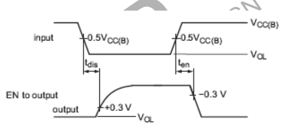
Figure 15. Enable and Disable Times
