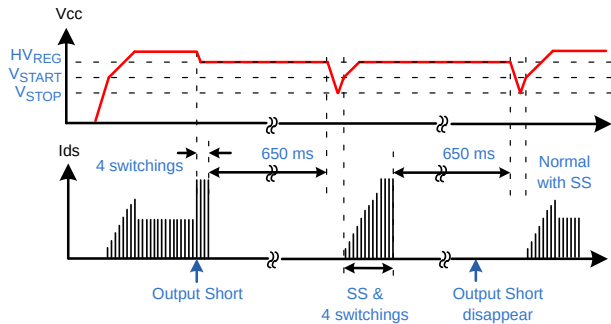
Figure 24. AOCP Waveform
