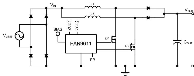
Figure 1. Simplified Application Diagram
