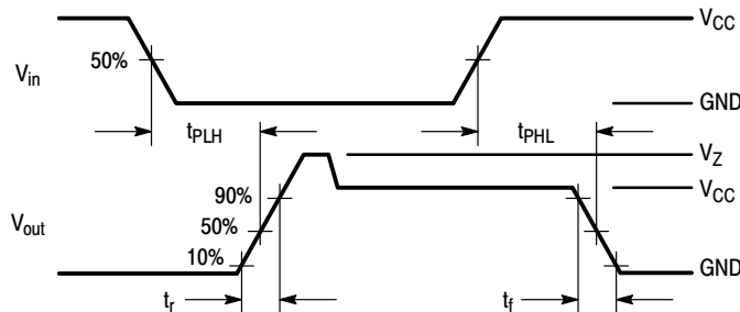
Figure 1. Switching Waveforms
