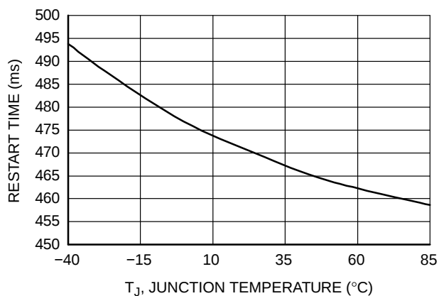
Figure 15. T_{RESTART} vs. Temperature
