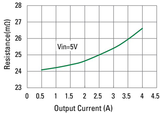
R_{ON} vs. Output Current
