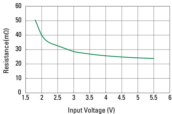
R_{ON} vs. Input Voltage
