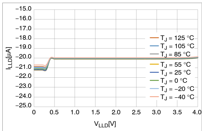
Figure 37. LLD Current
