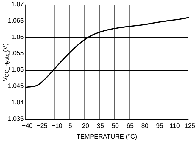
Figure 6. V_{CC} Hysteresis
