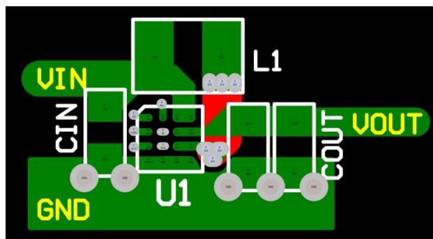
Figure 24. Layout Recommendation
