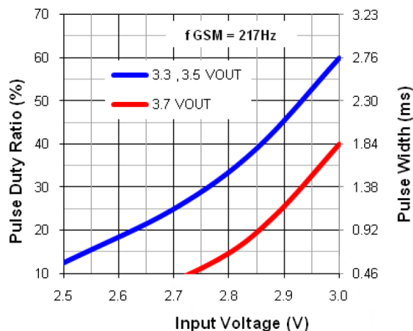
Figure 23. Minimum V IN for 2 A GSM Pulse, 3.5 V OUT
