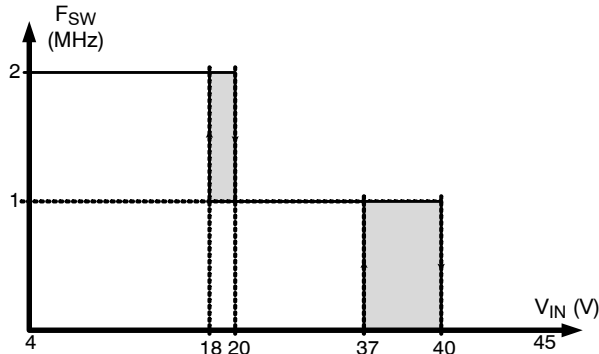
Figure 31. Switcher 1 Switching Frequency Reduction at High Input Voltage
