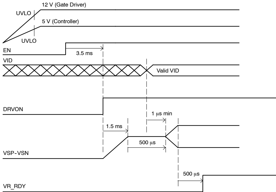
Figure 27. Normal Startup
