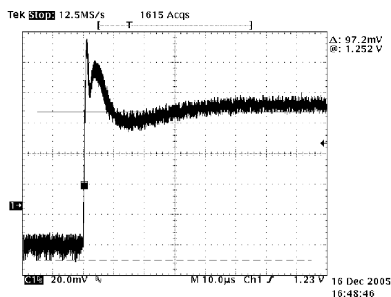
Figure 20. Typical Load Release Event
