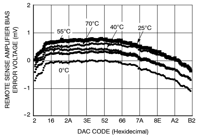
Figure 16. Remote Sense Amplifier Bias Error Voltage vs. DAC CODE
