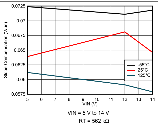
Figure 7-68. Slope Compensation Variation
