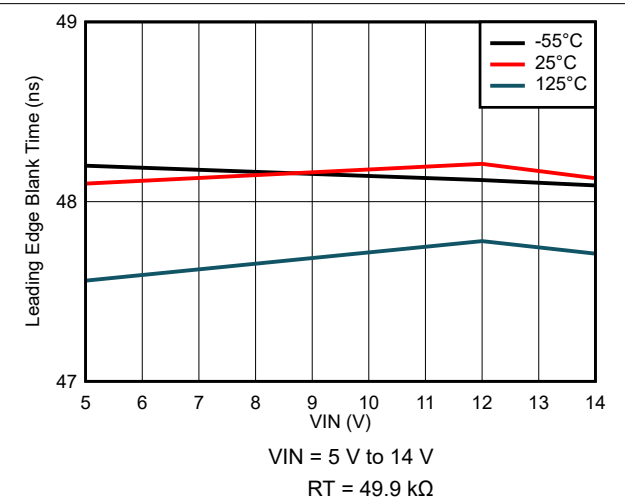
Figure 7-36. Leading Edge Blank Time Variation
