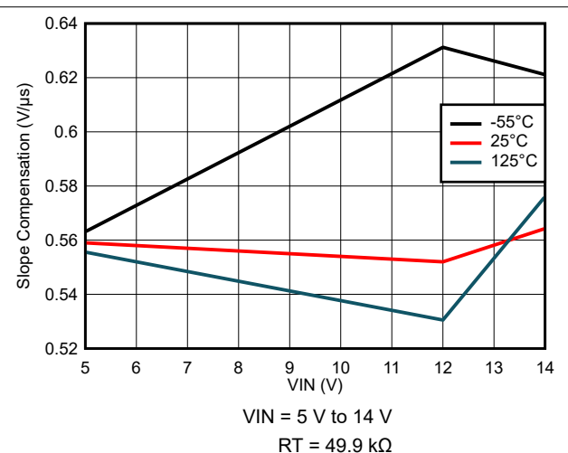
Figure 7-72. Slope Compensation Variation
