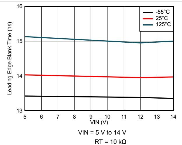
Figure 7-34. Leading Edge Blank Time Variation
