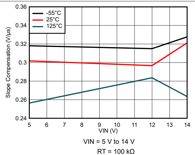
Figure 7-70. Slope Compensation Variation
