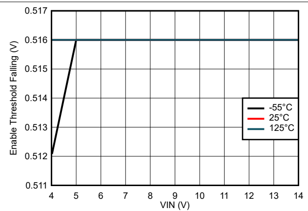
Figure 7-8. Enable Threshold Falling Variation
