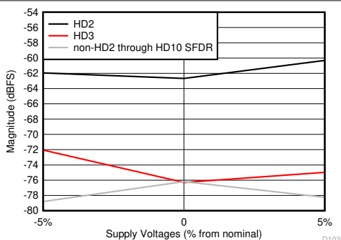
Figure 7-61. HD2, HD3 and Worst non-HD Spur vs Supply Voltage
