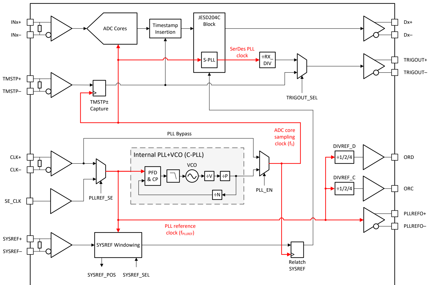
Figure 8-3. Clocking Subsystem
