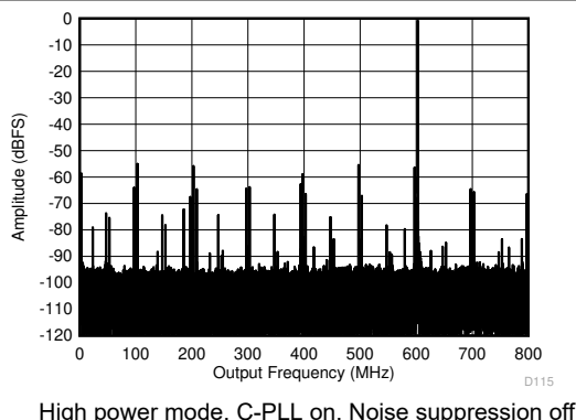
Figure 7-9. Single Tone FFT at 997 MHz and -1 dBFS
