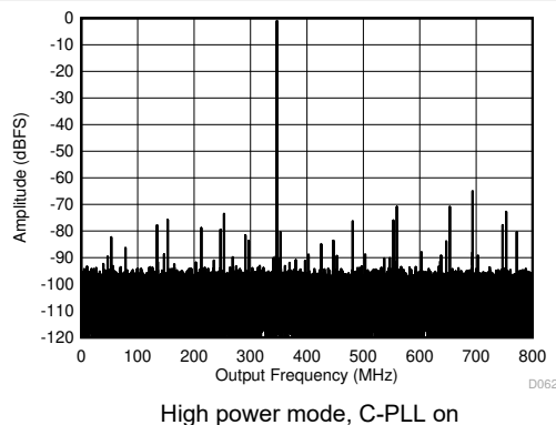
Figure 7-5. Single Tone FFT at 347 MHz and -1 dBFS
