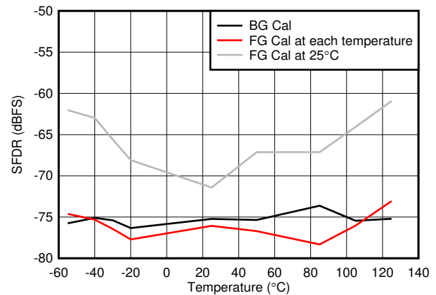
Figure 7-68. Worst Spur vs Temperature
