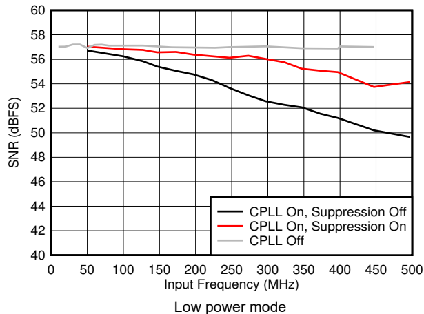
Figure 7-45. SNR vs F_{IN} and C-PLL modes
