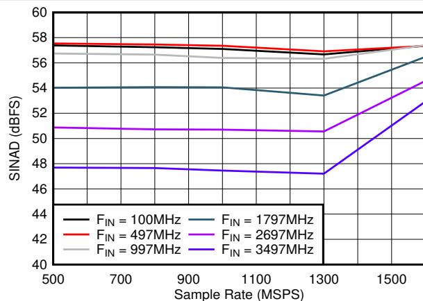
Figure 7-25. SINAD vs Sample Rate
