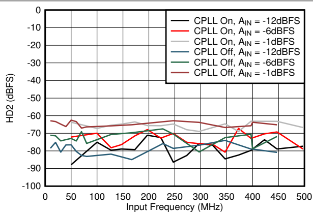
Figure 7-58. HD2 vs A_{IN} and C-PLL
