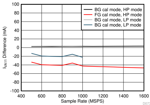
Figure 7-115. Quad Channel, I_{VA11} Change with Calibration Mode
