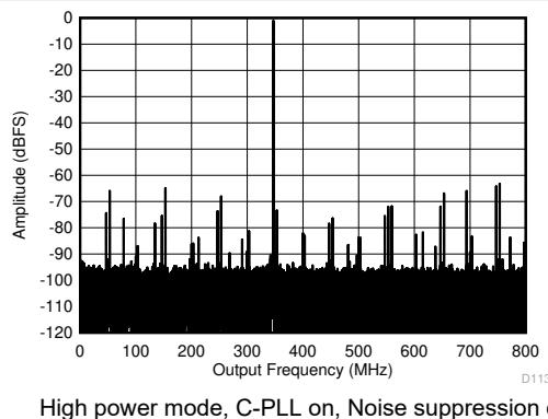
Figure 7-6. Single Tone FFT at 347 MHz and -1 dBFS
