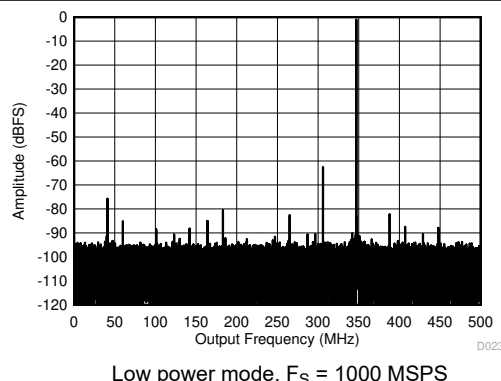
Figure 7-12. Single Tone FFT at 347 MHz and -1 dBFS
