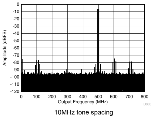
Figure 7-69. Two Tone FFT at 498MHz
