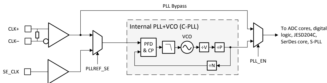
Figure 8-4. Converter PLL (C-PLL) Architecture
