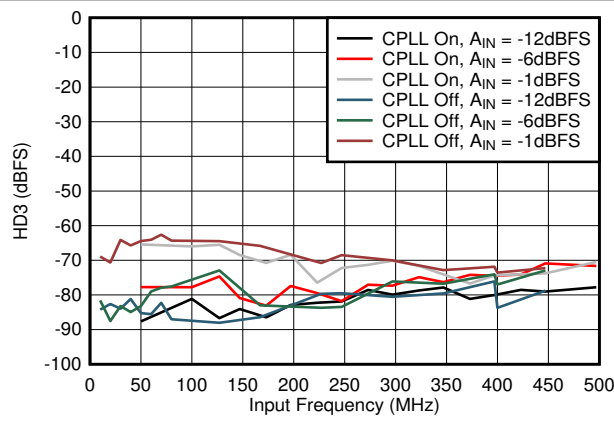
Figure 7-59. HD3 vs A_{IN} and C-PLL
