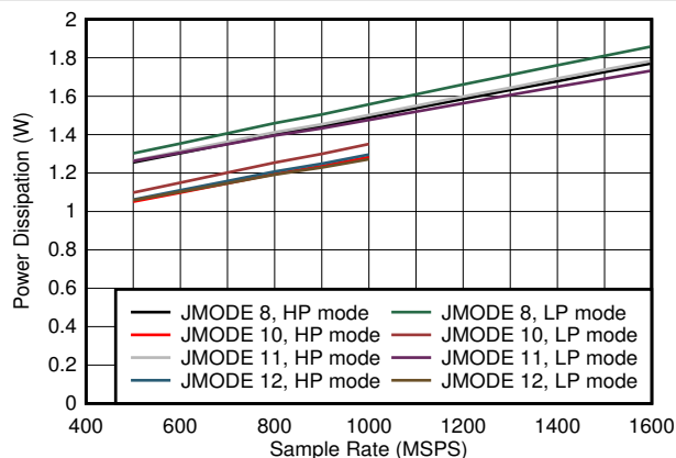
Figure 7-91. Dual Channel, Power Dissipation vs F_S and JMODE 8 - 12
