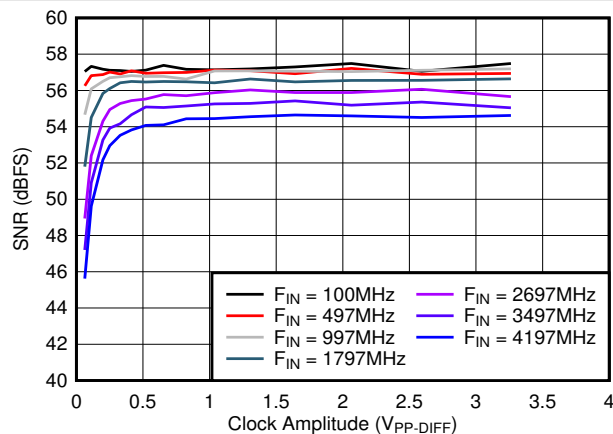
Figure 7-37. SNR vs A_{CLK}
