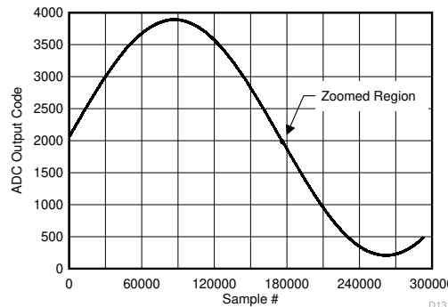
Figure 7-126. Background Calibration Core Transition (AC Signal)
