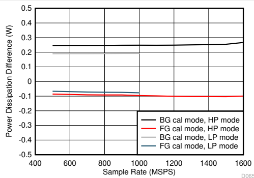
Figure 7-109. Quad Channel, Power Dissipation Change with Calibration Mode
