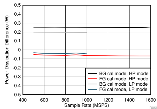
Figure 7-110. Dual Channel, Power Dissipation Change with Calibration Mode
