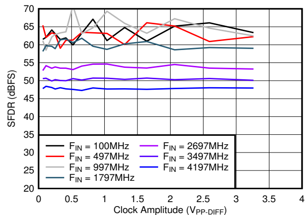
Figure 7-36. SFDR vs A_{CLK}
