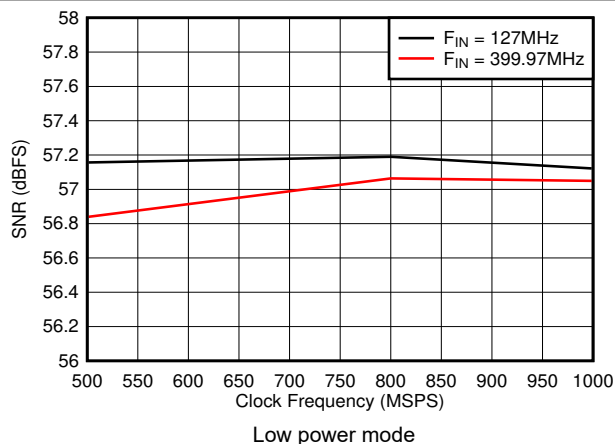
Figure 7-28. SNR vs Sample Rate
