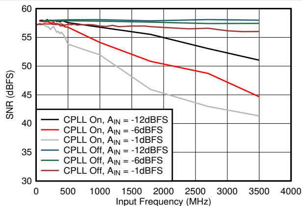
Figure 7-49. SNR vs A_{IN} and C-PLL
