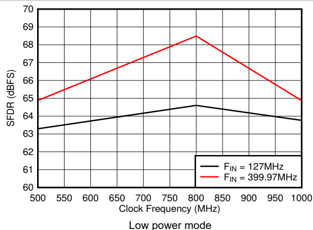
Figure 7-27. SFDR vs Sample Rate
