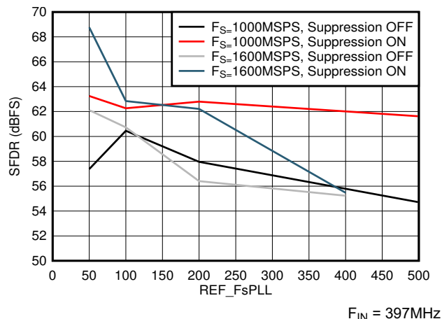
Figure 7-39. SFDR vs F_{REF} and Suppression
