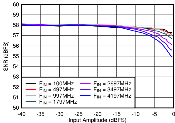
Figure 7-33. SNR vs A_{IN}
