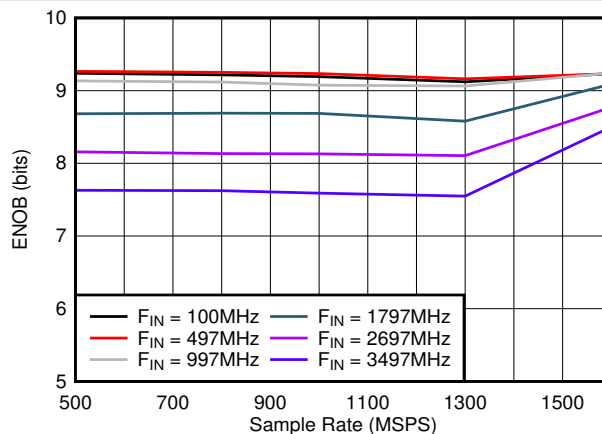
Figure 7-26. ENOB vs Sample Rate
