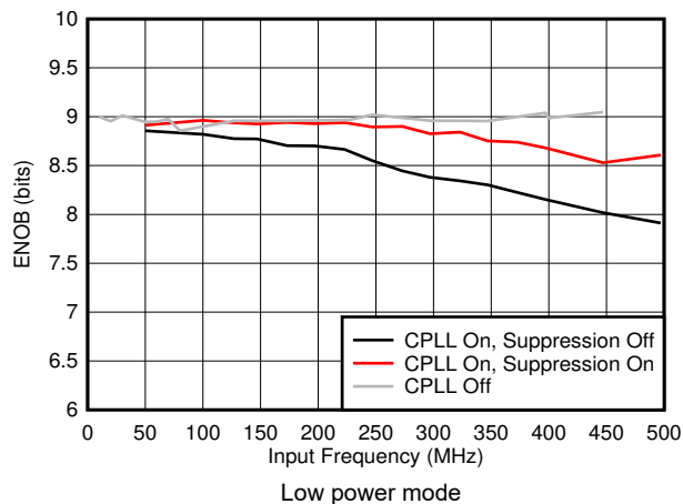
Figure 7-47. ENOB vs F_{IN} and C-PLL modes
