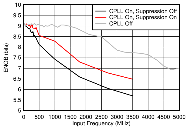
Figure 7-43. ENOB vs F_{IN} and C-PLL modes
