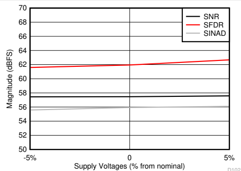
Figure 7-62. SNR, SFDR and SINAD vs Supply Voltages
