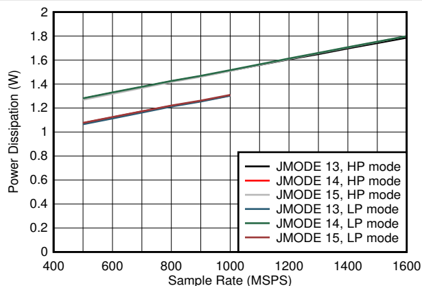
Figure 7-92. Dual Channel, Power Dissipation vs F_S and JMODE 13 - 15
