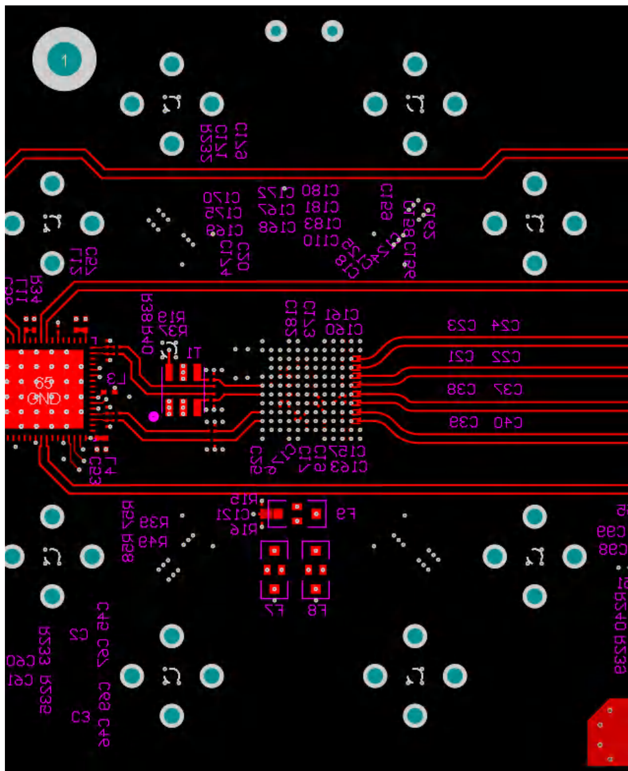
Figure 9-7. Bottom Layer Routing: CLK±, SYSREF and D[7:4]± Routing
