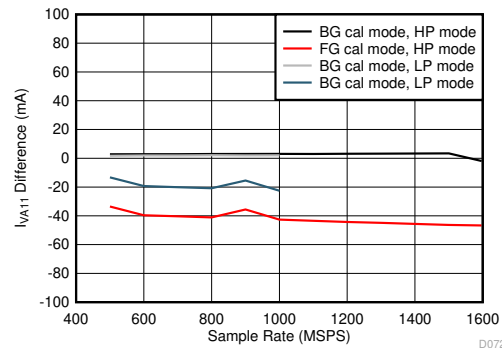
Figure 7-116. Dual Channel, I_{VA11} Change with Calibration Mode
