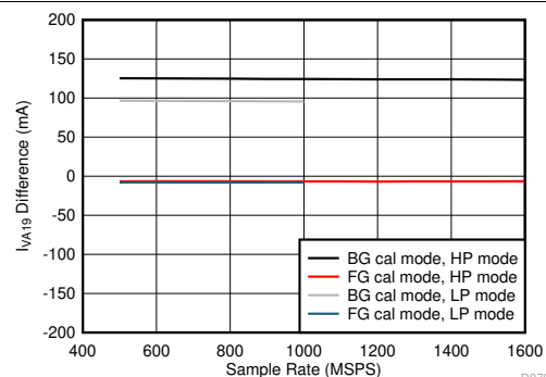
Figure 7-112. Quad Channel, I_{VA19} Change with Calibration Mode
