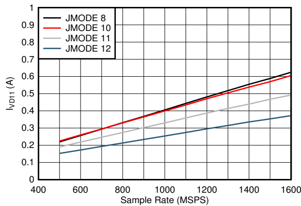
Figure 7-87. Quad Channel, I_{VD11} vs F_S and JMODE 8 - 12
