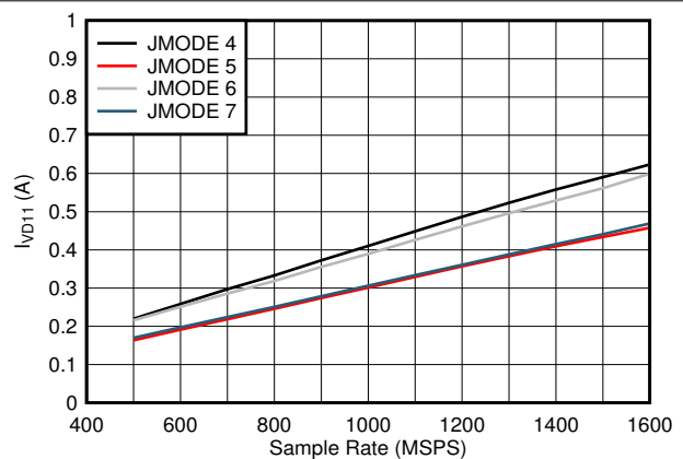
Figure 7-84. Quad Channel, I_{VDD11} vs F_S
