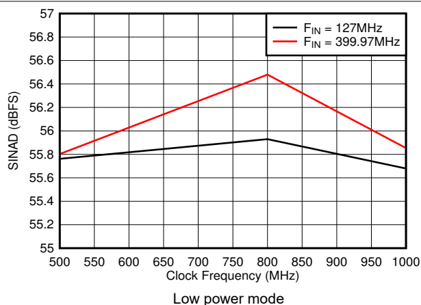
Figure 7-30. SINAD vs Sample Rate
