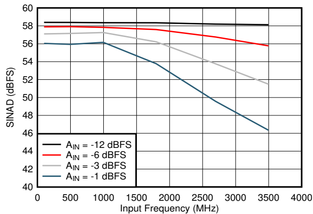
Figure 7-19. SINAD vs Input Frequency
