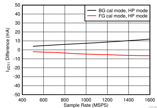
Figure 7-118. Quad Channel, I_{VD11} Change with Calibration Mode
