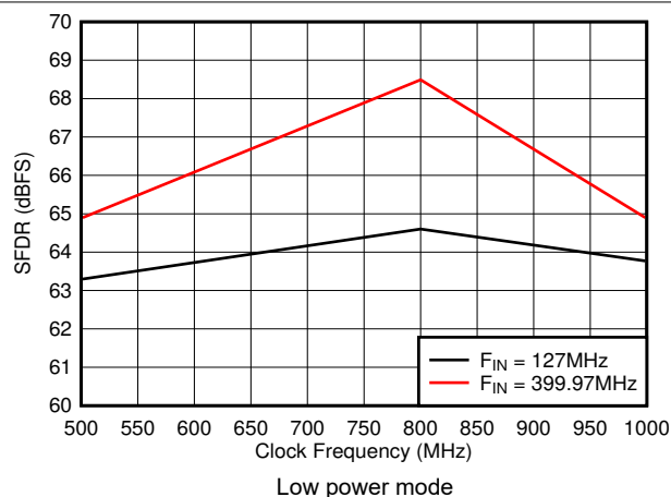
Figure 7-29. SFDR vs Sample Rate
