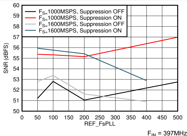
Figure 7-38. SNR vs F_{REF} and Suppression
