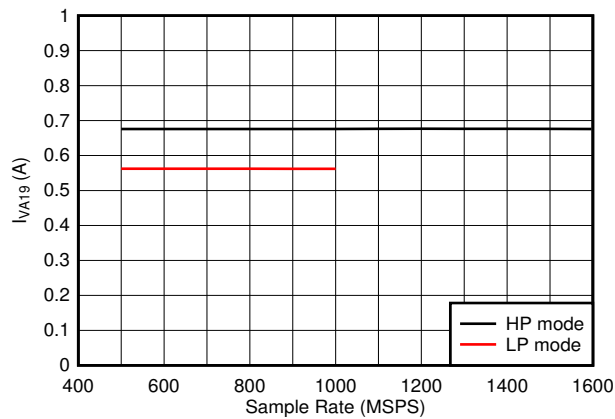
Figure 7-83. Quad Channel, I_{VA19} vs F_S
