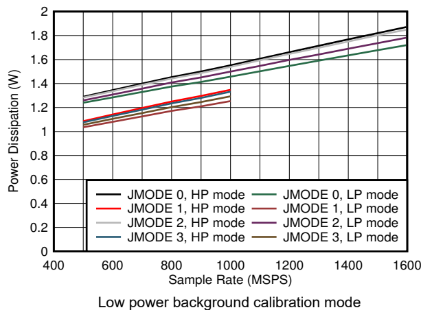
Figure 7-89. Dual Channel, Power Dissipation vs F_S and JMODE 0 - 3
