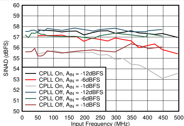
Figure 7-56. SINAD vs A_{IN} and C-PLL
