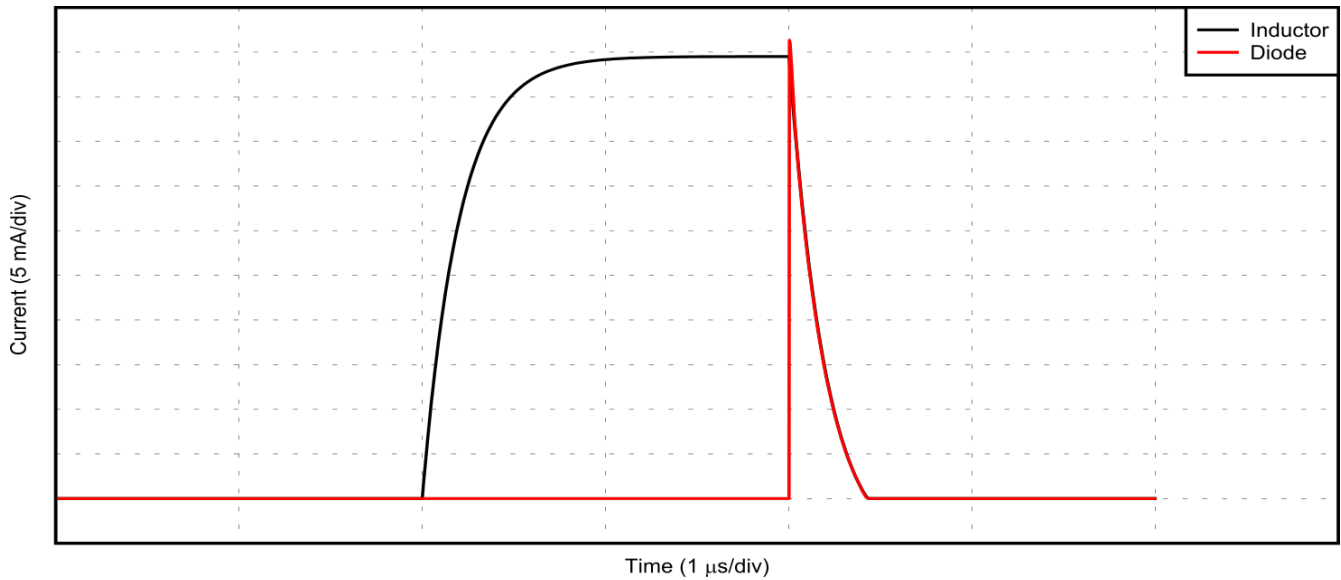
Figure 8-2. Application Curve
