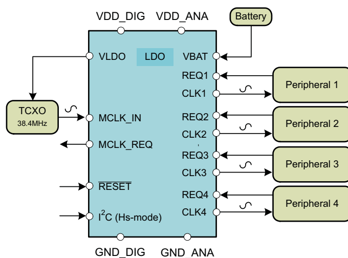
Figure 28. Clock Distribution Scheme
