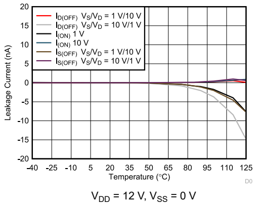
Figure 5-13. Leakage Current vs Temperature
