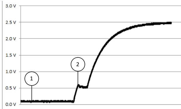
Figure 7-2. B-side Pedestal
