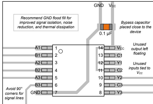
Figure 8-3. Example Layout for the SN54SC3T97-SEP
