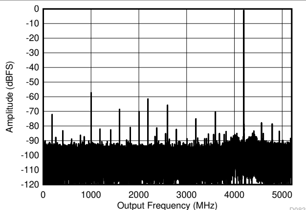
Figure 5-8. DES Mode: Single Tone FFT at 4197 MHz
