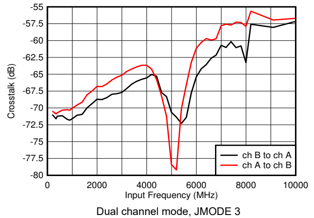
Figure 5-2. Crosstalk vs Input Frequency
