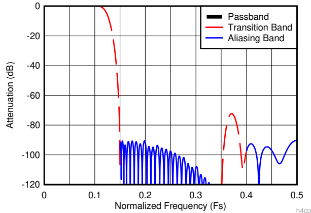
Figure 6-11. Decimate-by-4 Composite Response
