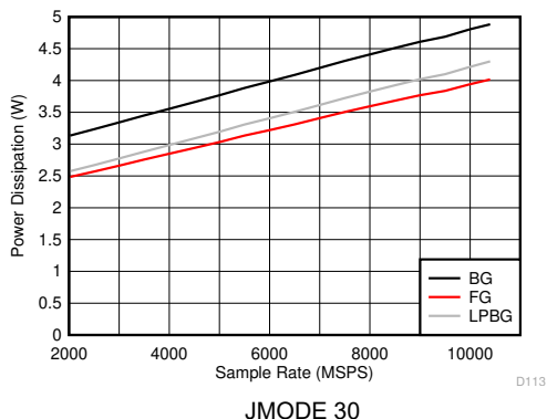
Figure 5-131. DES Mode: Power Dissipation vs Sample Rate
