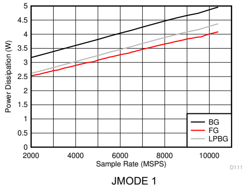
Figure 5-129. DES Mode: Power Dissipation vs Sample Rate
