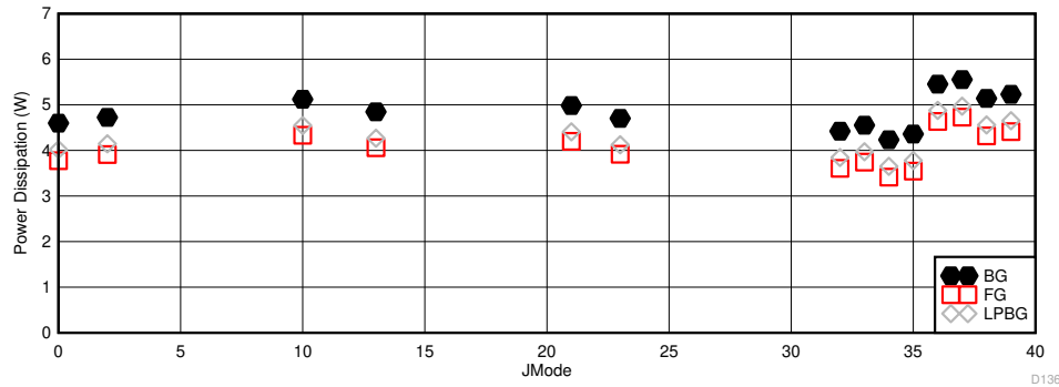
Figure 5-122. Other Modes with Lower Maximum F_S : Power Dissipation vs JMODE
