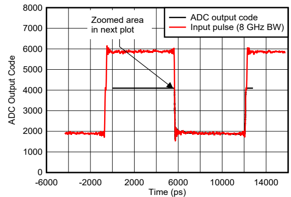
Figure 5-148. Pulse Overdrive Recovery
