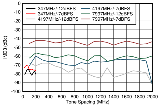
Figure 5-103. DES Mode: IMD3 vs Tone Spacing
