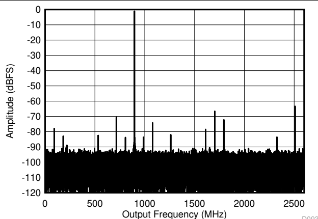
Figure 5-18. Dual Channel Mode: Single Tone FFT at 897 MHz
