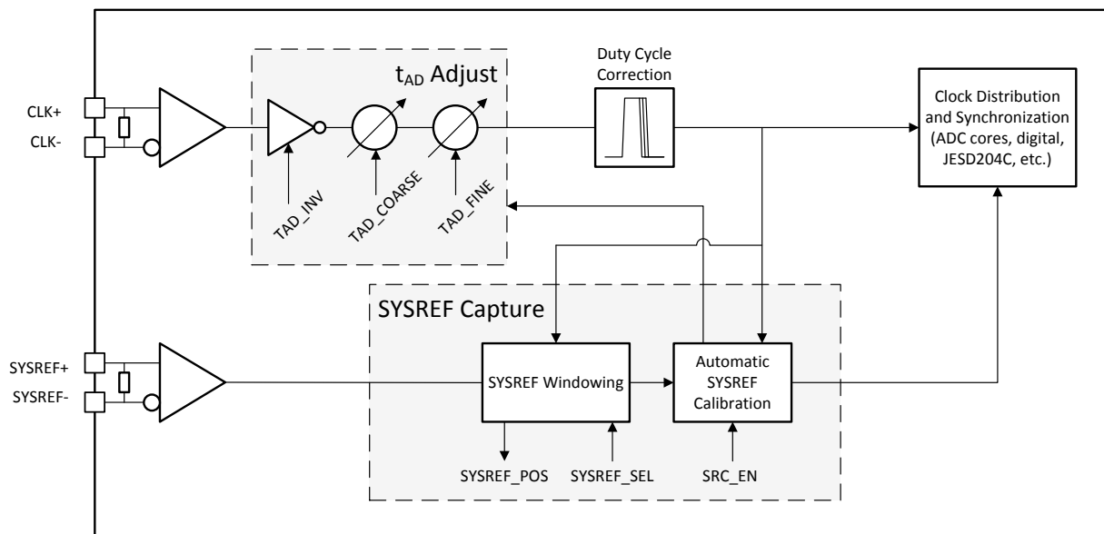
Figure 6-2. Clocking Subsystem
