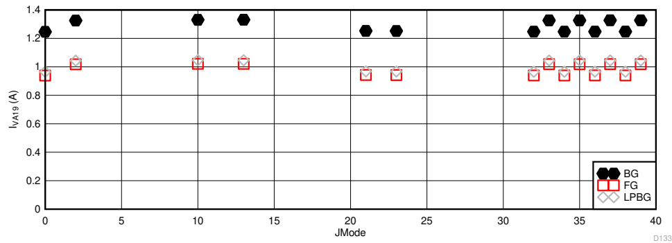
Figure 5-119. Other Modes with Lower Maximum F_S : I_{VA19} vs JMODE
