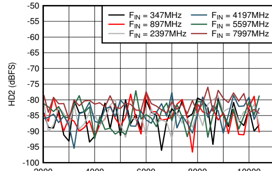
Figure 5-38. DES Mode: HD2 vs Sample Rate and Input Frequency
