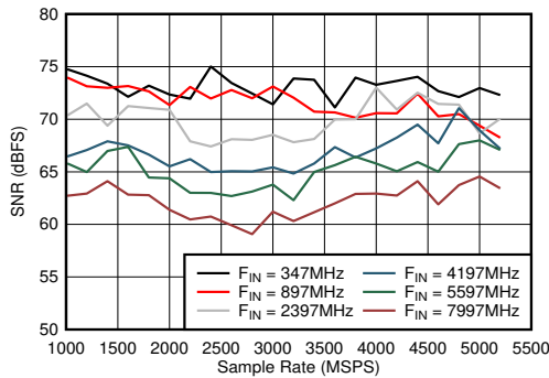
Figure 5-49. Dual Channel Mode: SNR vs Sample Rate and Input Frequency
