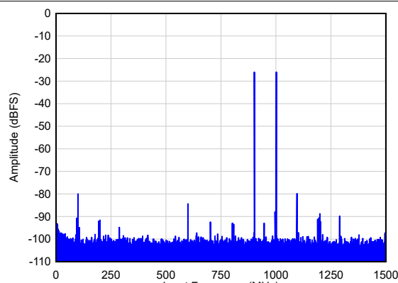
Figure 6-80. Two Tone FFT at F_{IN} = 900/1000 MHz
