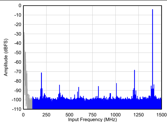
Figure 6-63. Single Tone FFT at F_{IN} = 1400 MHz
