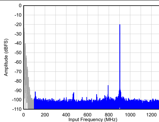
Figure 6-20. Single Tone FFT at F_{IN} = 900 MHz
