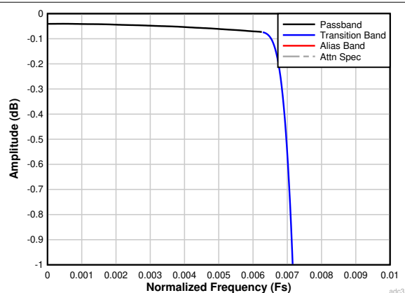
Figure 7-34. Decimation by 64 Passband Ripple Response
