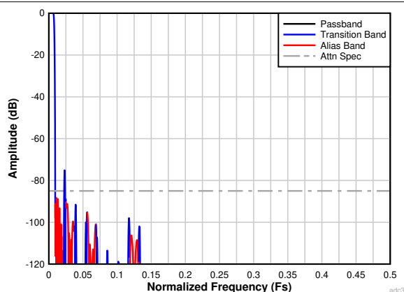
Figure 7-32. Complex Decimation by 64 Filter Response
