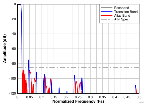
Figure 7-30. Complex Decimation by 32 Filter Response
