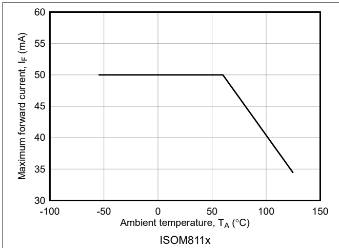
Figure 7-1. Maximum Forward Current vs Ambient Temperature
