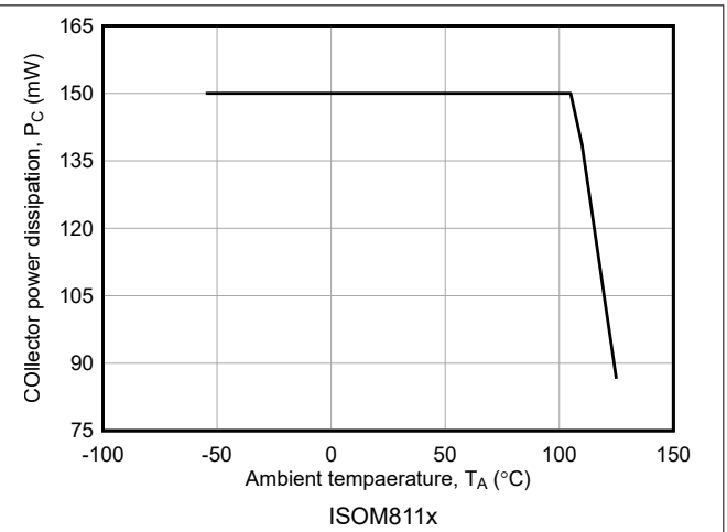
Figure 7-2. Maximum Collector Power Dissipation vs Ambient Temperature
