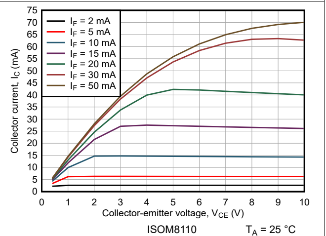
Figure 7-4. Collector Current vs Collector-Emitter Voltage
