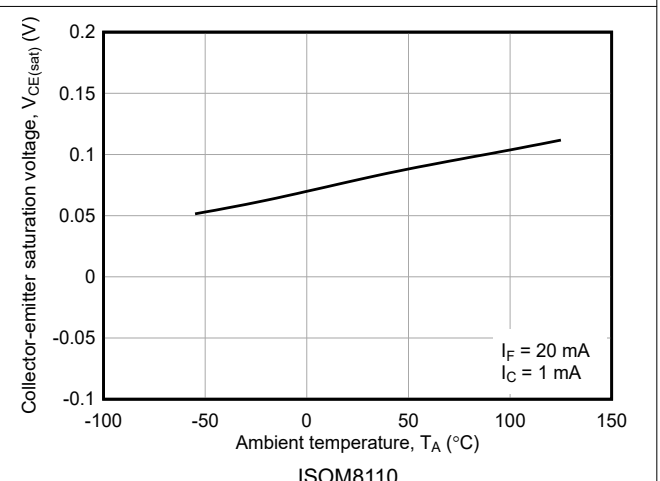
Figure 7-6. Collector-Emitter Saturation Voltage vs Ambient Temperature
