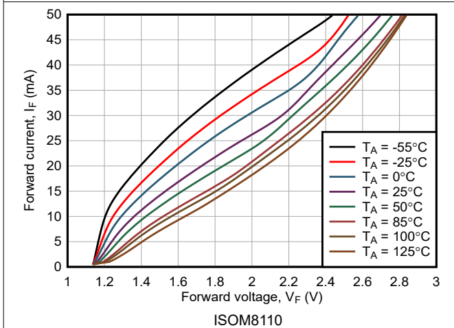
Figure 7-3. Forward Voltage vs Forward Current
