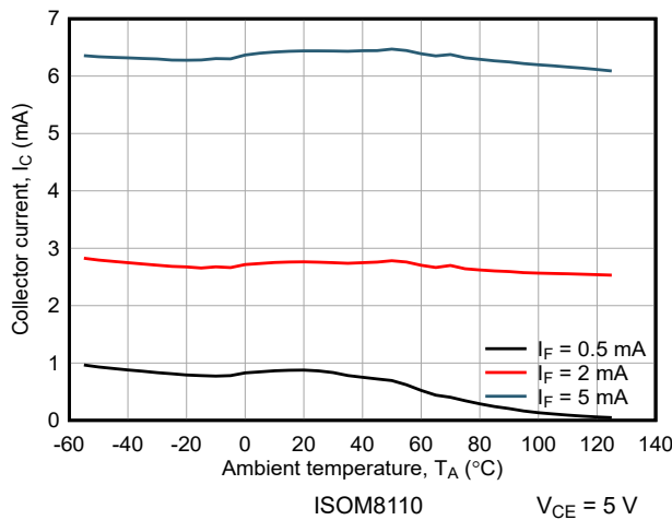
Figure 7-9. Collector Current vs Ambient Temperature
