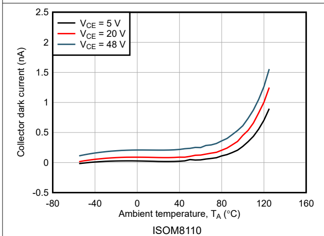
Figure 7-5. Collector Dark Current vs Ambient Temperature
