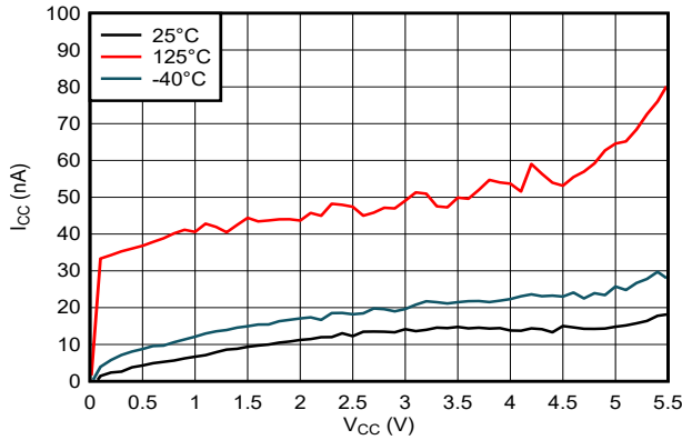
Figure 5-1. Supply Current Across Voltage Supply Voltage
