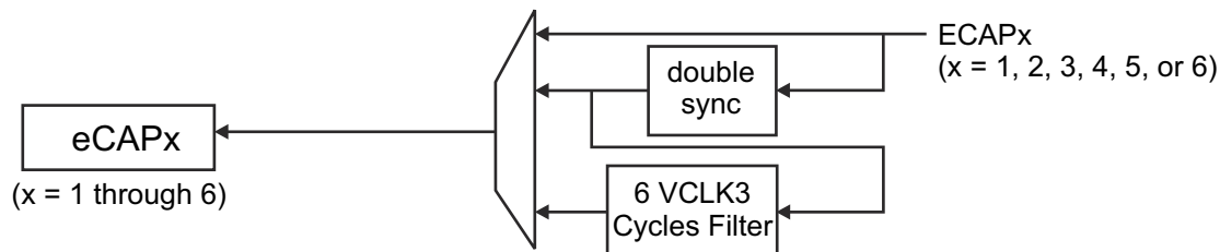
Figure 8-6. eCAPx Input Synchronization Selection Detail
