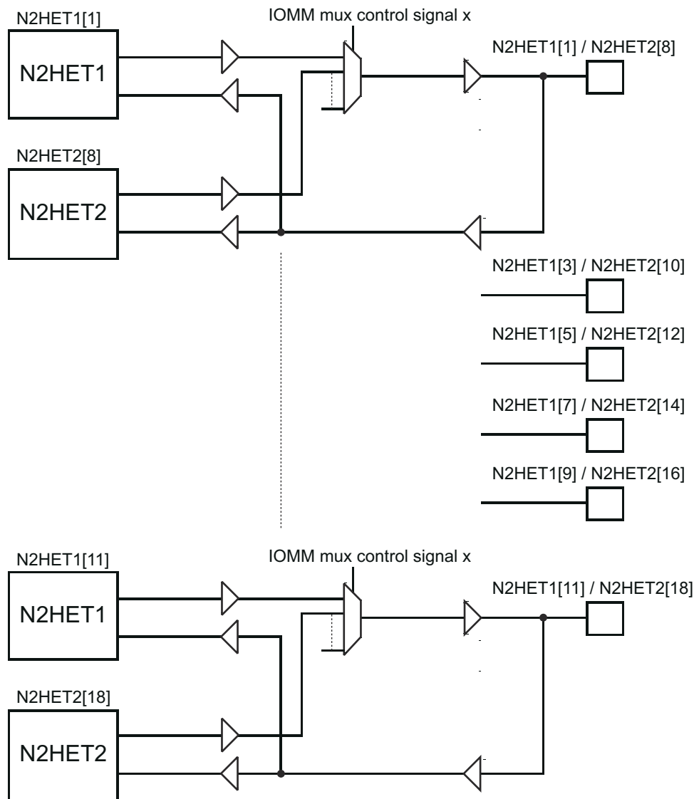
Figure 8-17. N2HET Monitoring
