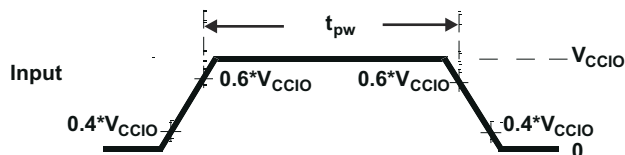
Figure 6-4. FlexRay Inputs
