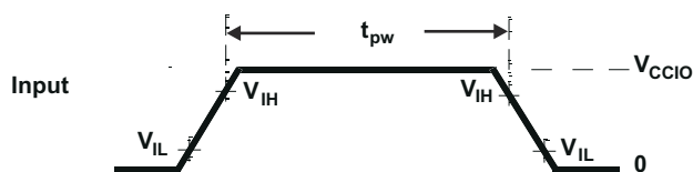
Figure 6-3. TTL-Level Inputs
