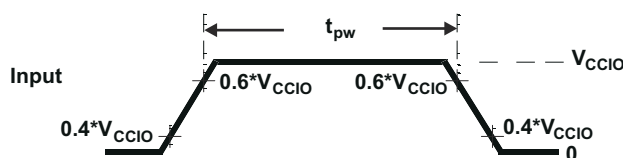
Figure 8-18. FlexRay Inputs
