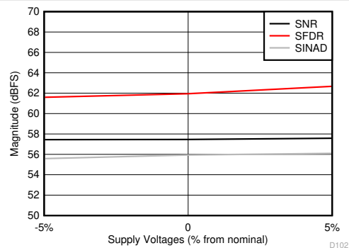
Figure 7-62. SNR, SFDR and SINAD vs Supply Voltages
