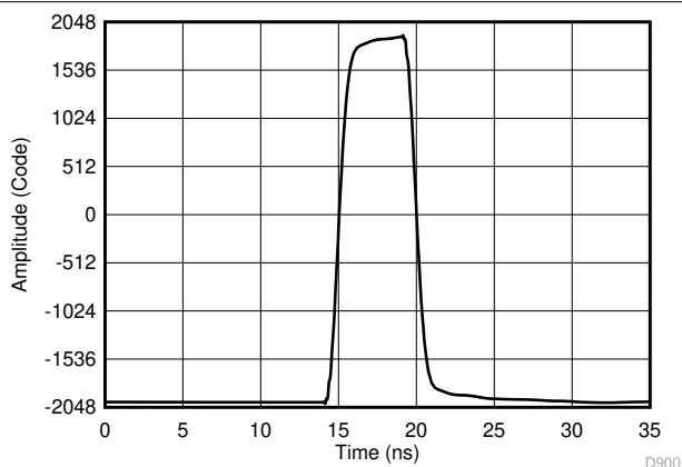
Figure 9-2. Measured Pulse using Sub-Sampling Technique for Equivalent 32 GSPS Measurement
