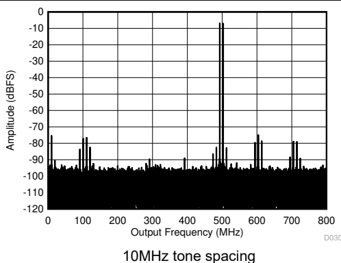
Figure 7-69. Two Tone FFT at 498MHz
