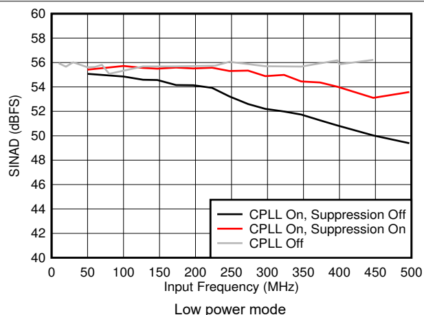
Figure 7-46. SINAD vs F_{IN} and C-PLL modes
