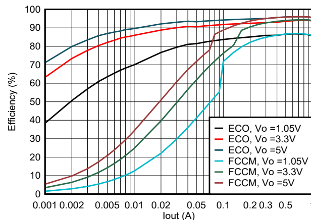
TPS56124x Efficiency at Vin = 12V
