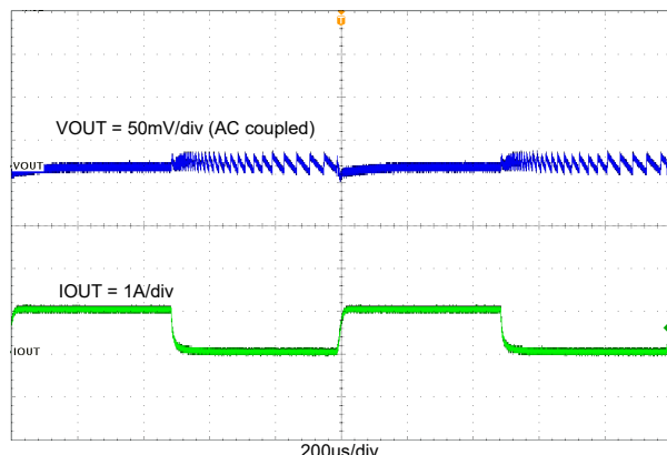
Figure 7-14. TPS561243 Load Transient With 0A to 1A
