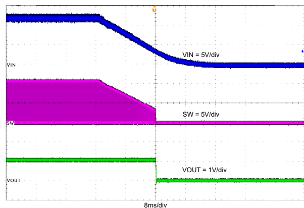
Figure 7-13. TPS561246 Power Off With 1A Loading
