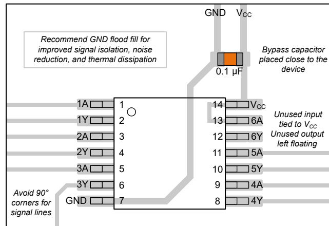
Figure 8-3. Example Layout for the SN54SC6T07-SEP
