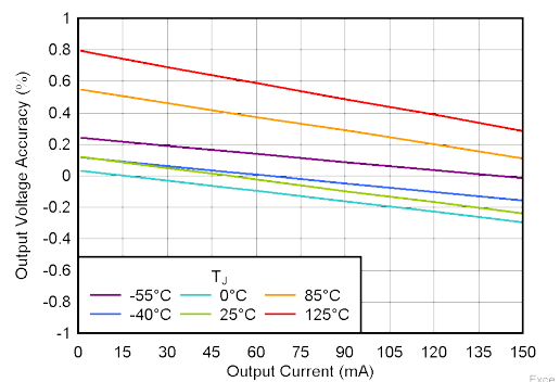
Figure 5-2. Load Regulation vs I_{OUT}
