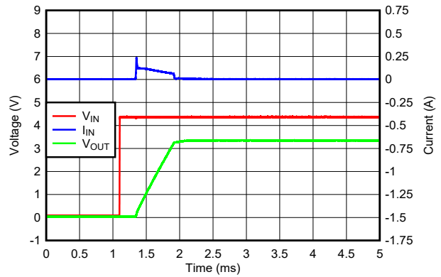
Figure 5-20. Inrush Current With 22\text{ }\mu\text{F} at C_{OUT}
