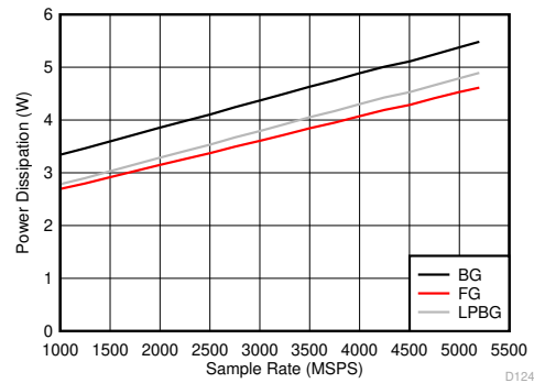
Figure 6-140. Dual Channel Mode: Power Dissipation vs Sample Rate
