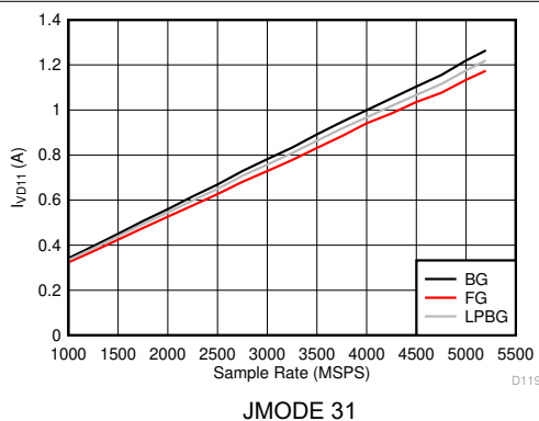
Figure 6-137. Dual Channel Mode: I_{VD11} vs Sample Rate
