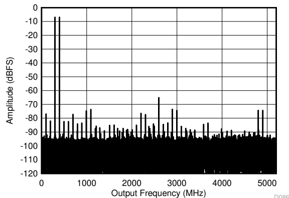
each tone at -7 dBFS, 100MHz Tone Spacing Figure 6-11. DES Mode: Two Tone FFT at 347 MHz
