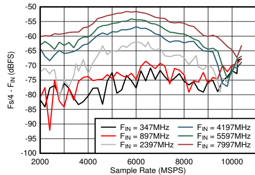
Figure 6-44. DES Mode: F_s/4 - F_{\text{IN}} vs Sample Rate and Input Frequency
