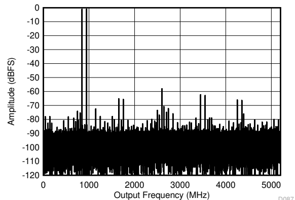
each tone at -7 dBFS, 100 MHz Tone Spacing Figure 6-12. DES Mode: Two Tone FFT at 897 MHz
