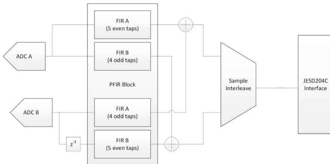
Figure 7-7. Alternate I/Q Correction-Type Filter Block Diagram
