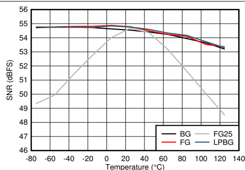
Figure 6-92. Dual Channel Mode: SNR vs Temperature and Calibration Mode
