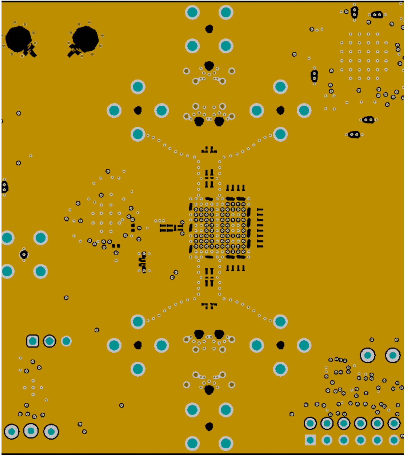
Figure 8-6. GND1 Cutouts to Optimize Impedance of Component Pads
