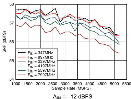
Figure 6-47. Dual Channel Mode: SNR vs Sample Rate and Input Frequency
