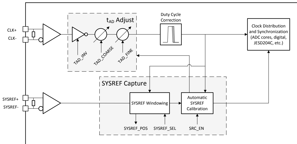
Figure 7-2. Clocking Subsystem
