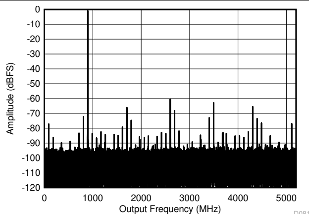
Figure 6-6. DES Mode: Single Tone FFT at 897 MHz
