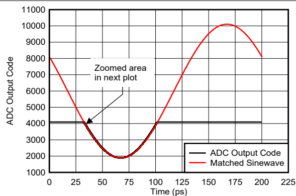
Figure 6-150. Sinewave Overdrive Recovery
