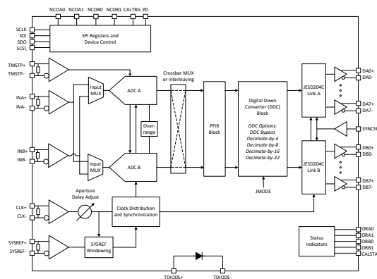
ADC12DJ5200-SP Block Diagram
