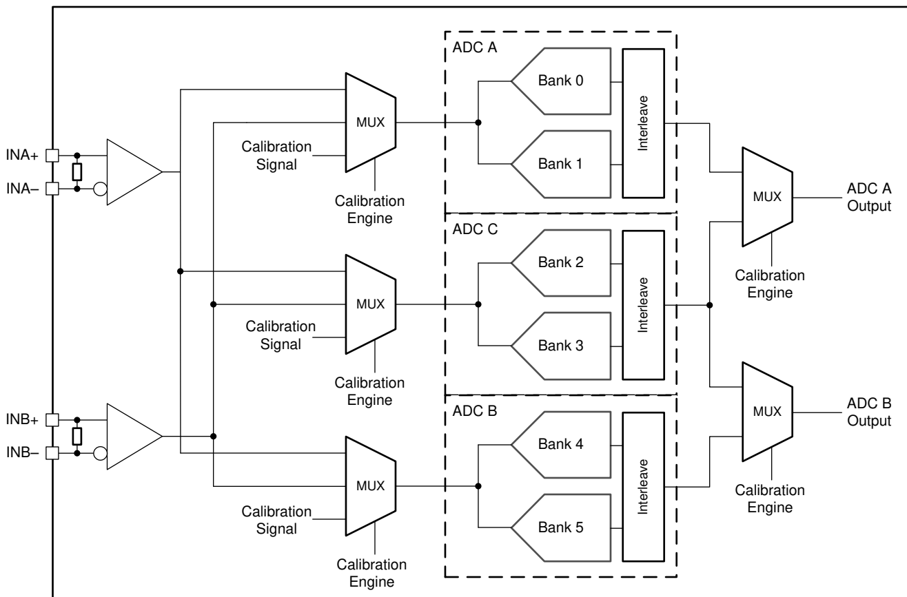
Figure 7-25. ADC12DJ5200-SP Calibration System Block Diagram
