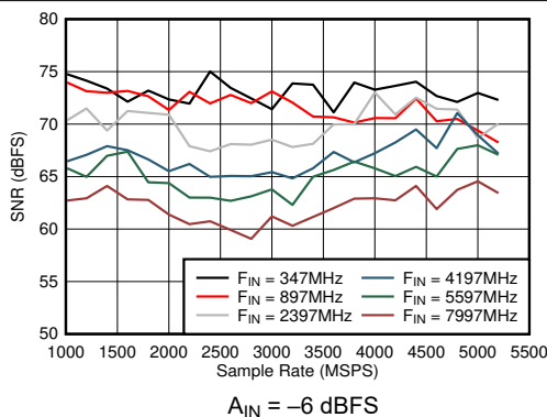
Figure 6-49. Dual Channel Mode: SNR vs Sample Rate and Input Frequency
