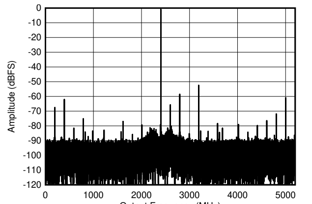
Figure 6-10. DES Mode: Single Tone FFT at 7997 MHz
