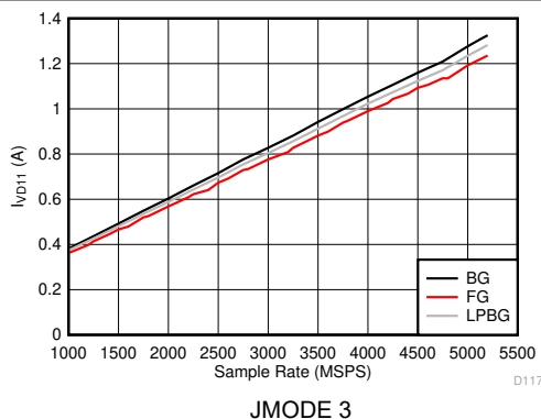
Figure 6-135. Dual Channel Mode: I_{VD11} vs Sample Rate
