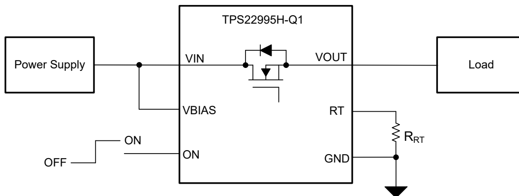
Figure 9-1. TPS22995H-Q1 Application Schematic
