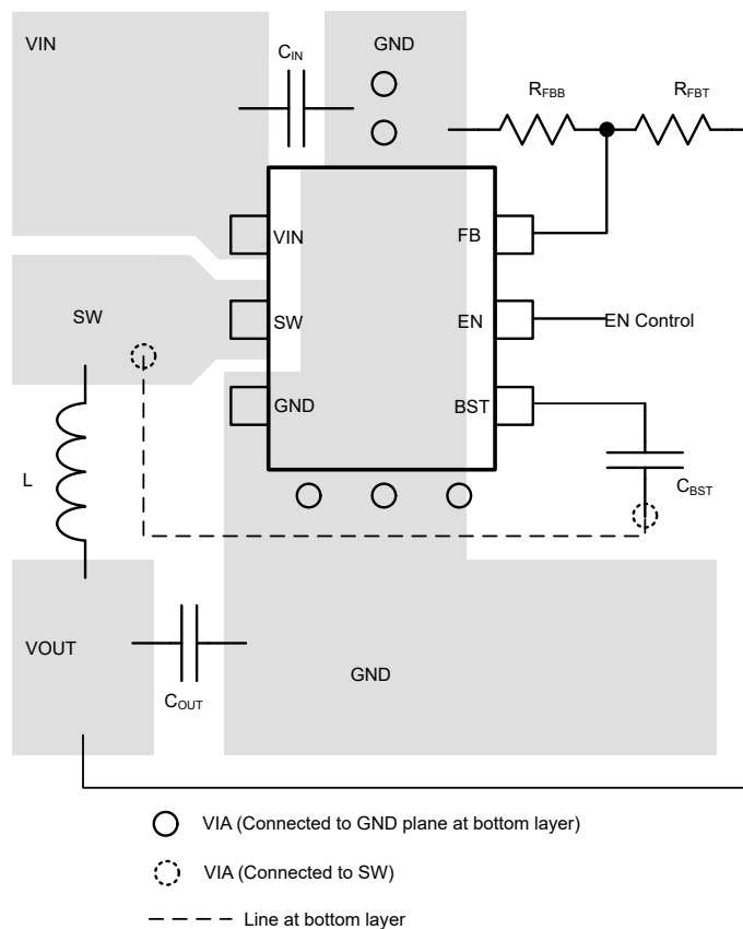
Figure 7-18. TPS56224x Layout
