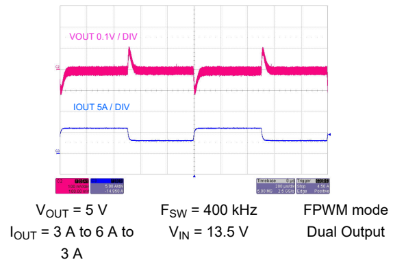
Figure 8-48. Load Transient
