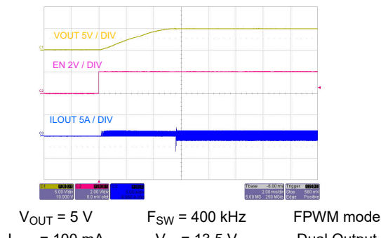
Figure 8-38. Start-Up With 100-mA Load
