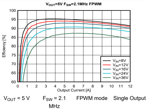
Figure 8-17. Efficiency
