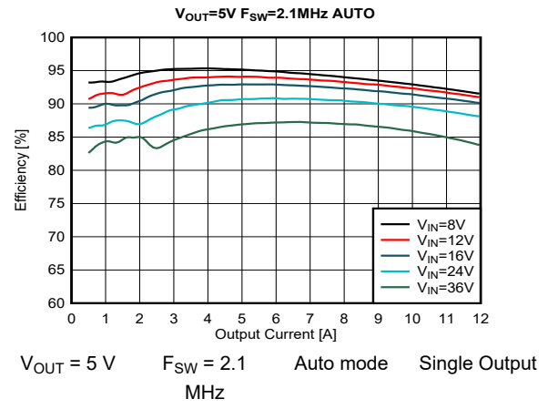
Figure 8-16. Efficiency
