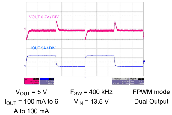
Figure 8-46. Load Transient
