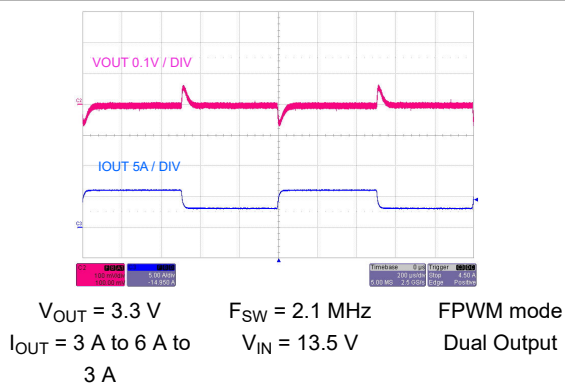
Figure 8-51. Load Transient
