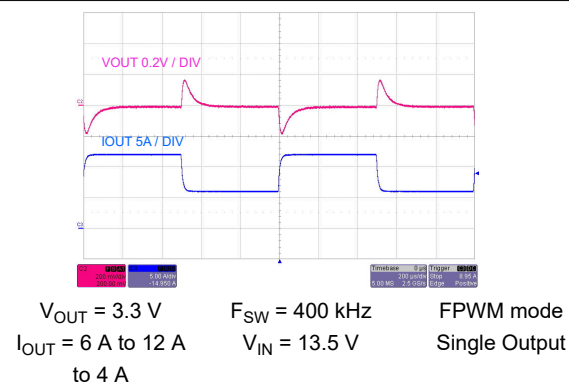
Figure 8-56. Load Transient
