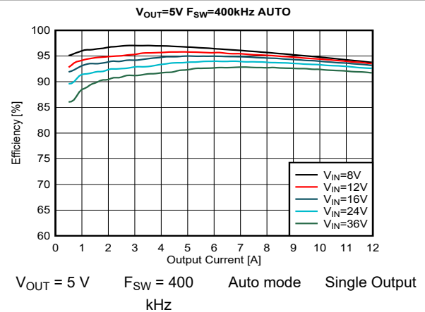
Figure 8-10. Efficiency
