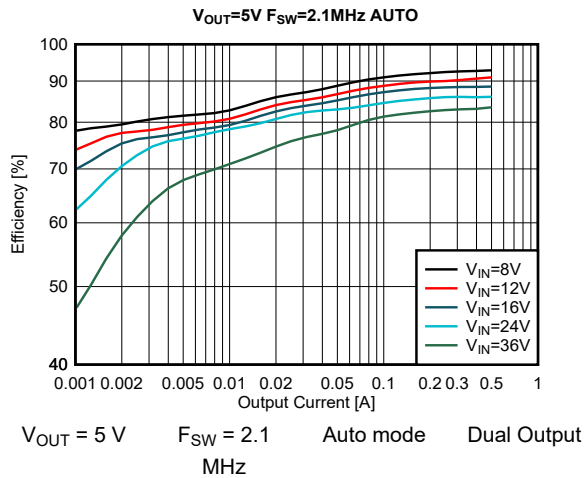
Figure 8-21. Efficiency
