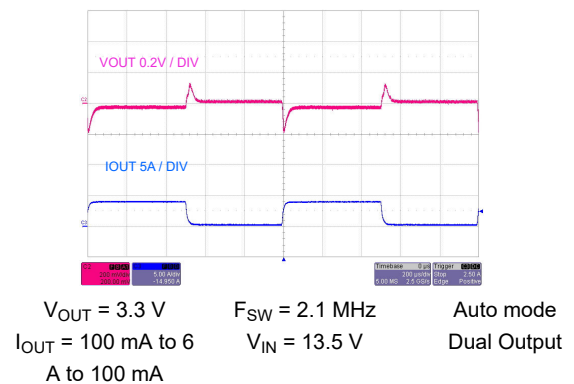
Figure 8-50. Load Transient
