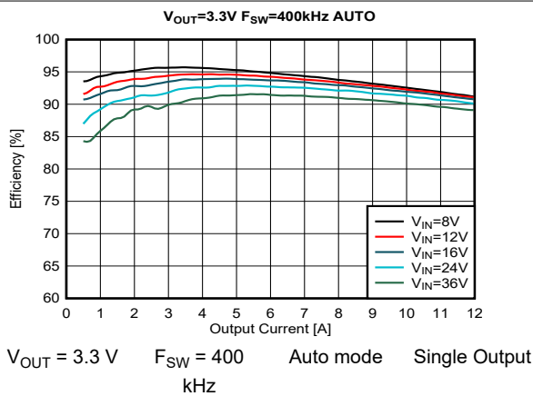
Figure 8-13. Efficiency
