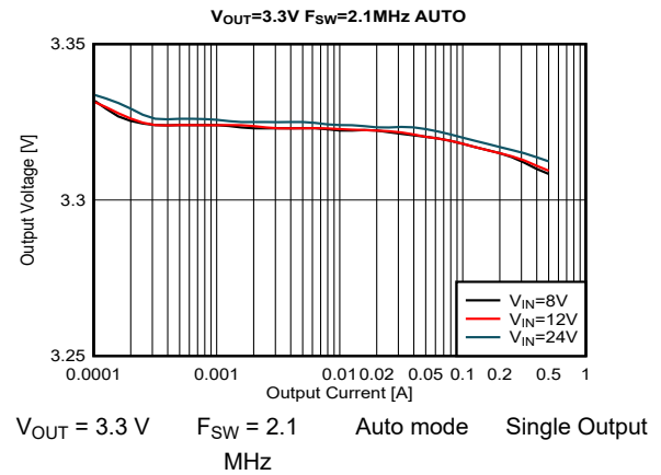
Figure 8-28. Load and Line Regulation
