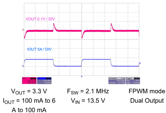
Figure 8-49. Load Transient
