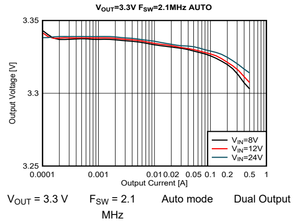
Figure 8-30. Load and Line Regulation
