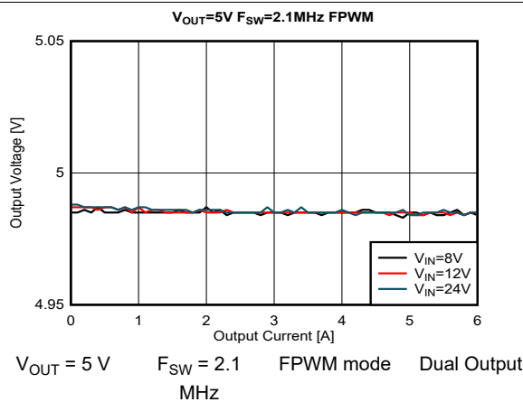
Figure 8-31. Load and Line Regulation
