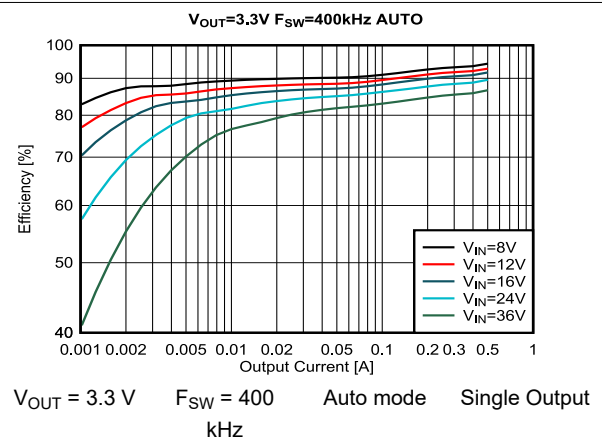
Figure 8-12. Efficiency
