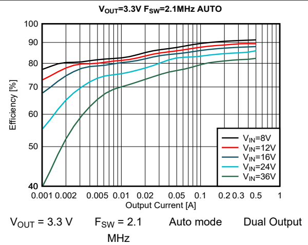
Figure 8-24. Efficiency
