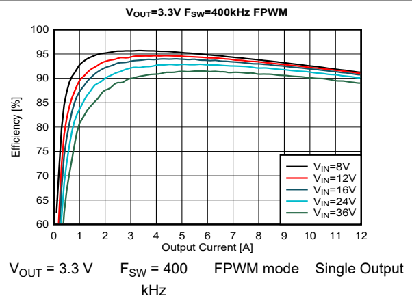
Figure 8-14. Efficiency
