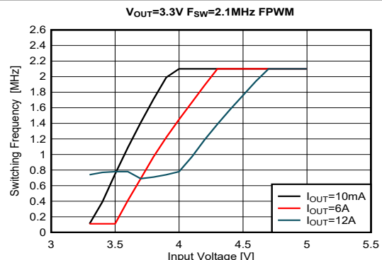
Figure 8-34. Dropout
