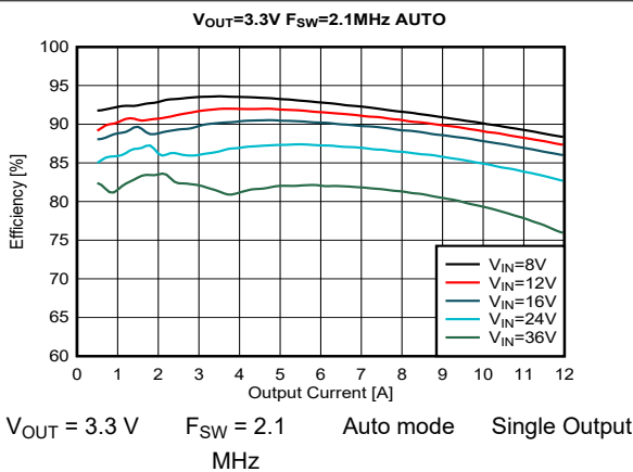
Figure 8-19. Efficiency
