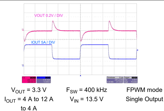
Figure 8-55. Load Transient
