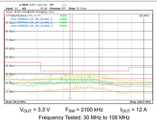
Figure 8-68. Dual Output Conducted Emissions versus CISPR25 Class 5 Limits (Orange: Peak Signal, Red: Average Signal, Green: Quasi-Peak Signal)
