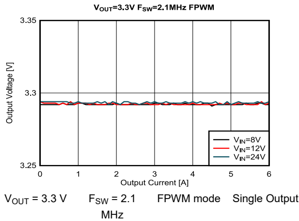
Figure 8-27. Load and Line Regulation
