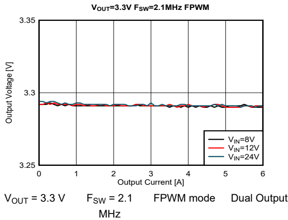
Figure 8-29. Load and Line Regulation
