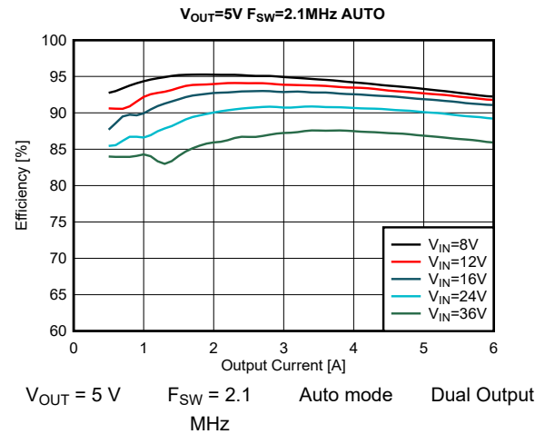
Figure 8-22. Efficiency
