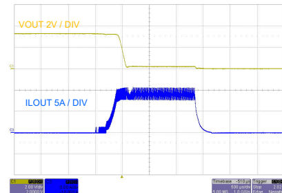
Figure 8-40. Start-Up With 12-A Load
