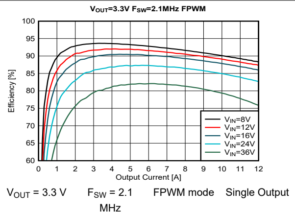
Figure 8-20. Efficiency
