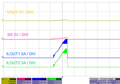
Figure 8-41. Short-Circuit Protection
