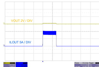
Figure 8-42. Short-Circuit Protection
