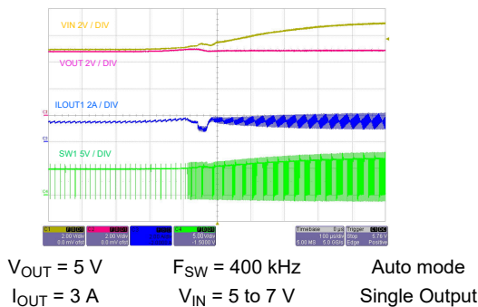
Figure 8-37. Dropout Recovery
