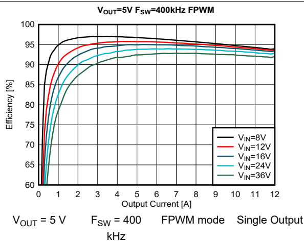
Figure 8-11. Efficiency
