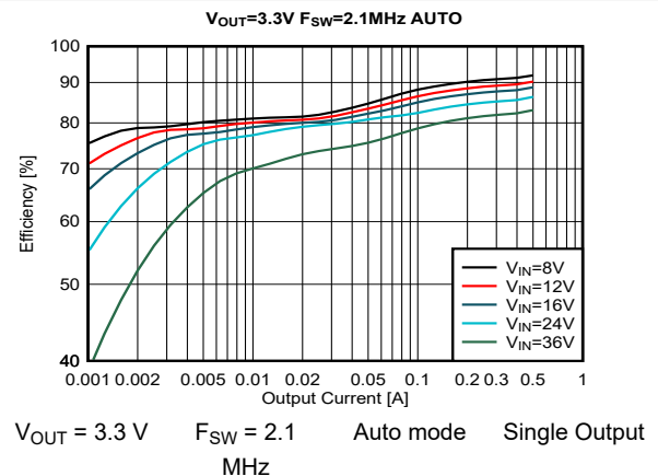
Figure 8-18. Efficiency
