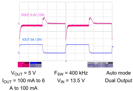
Figure 8-47. Load Transient
