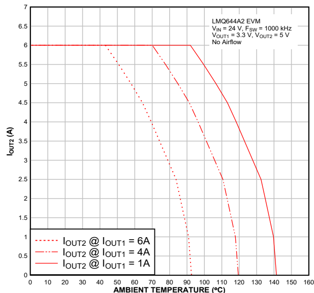
Figure 8-6. Typical Output Current versus Ambient Temperature, V_{IN} = 24\text{ V} F_{SW} = 1\text{ MHz} , Dual Output
