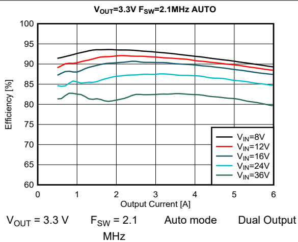
Figure 8-25. Efficiency
