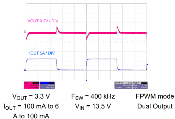
Figure 8-52. Load Transient
