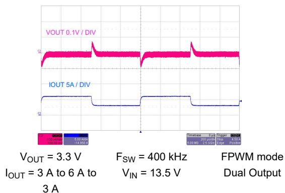
Figure 8-54. Load Transient
