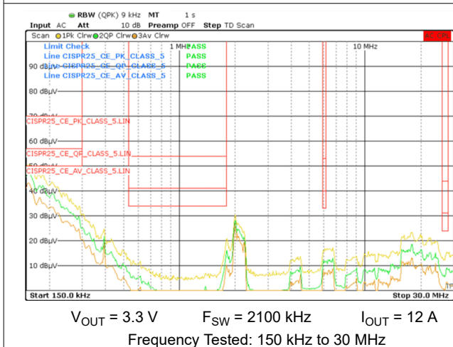
Figure 8-67. Dual Output Conducted Emissions versus CISPR25 Class 5 Limits (Orange: Peak Signal, Red: Average Signal, Green: Quasi-Peak Signal)
