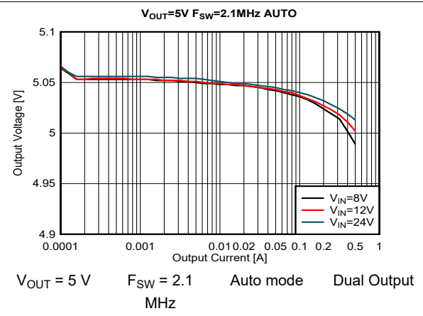
Figure 8-32. Load and Line Regulation
