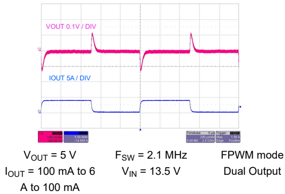
Figure 8-45. Load Transient
