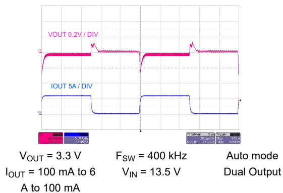
Figure 8-53. Load Transient
