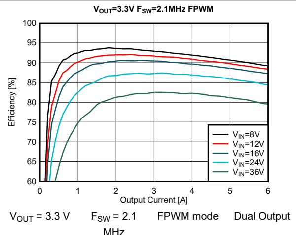
Figure 8-26. Efficiency
