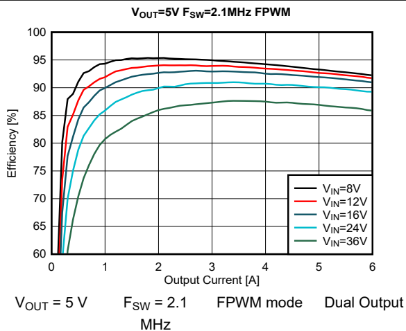
Figure 8-23. Efficiency
