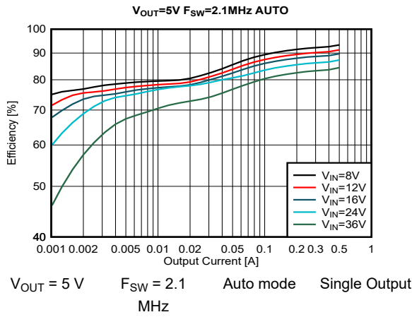
Figure 8-15. Efficiency
