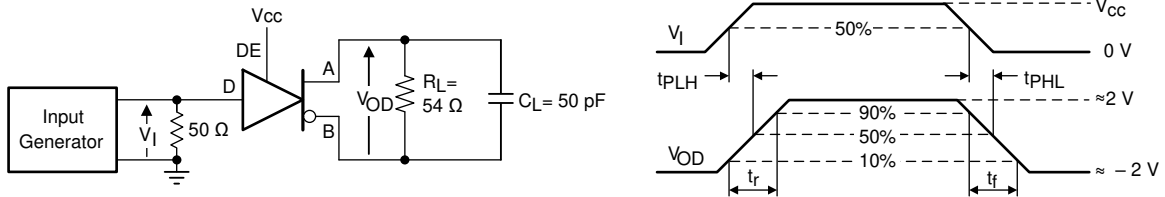
Figure 6-3. Measurement of Driver Differential Output Rise and Fall Times and Propagation Delays
