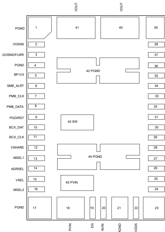
Figure 4-1. 45-Pin QFM-MOY Package (Top View)
