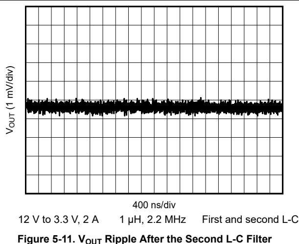
Figure 5-11. V_{OUT} Ripple After the Second L-C Filter
