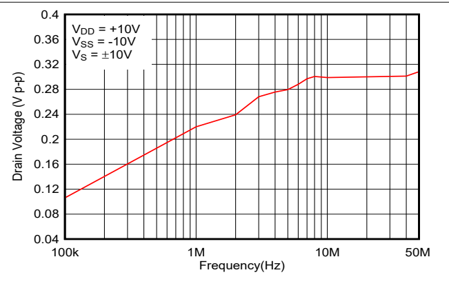
Figure 5-10. Large Signal Voltage Off Isolation vs Frequency
