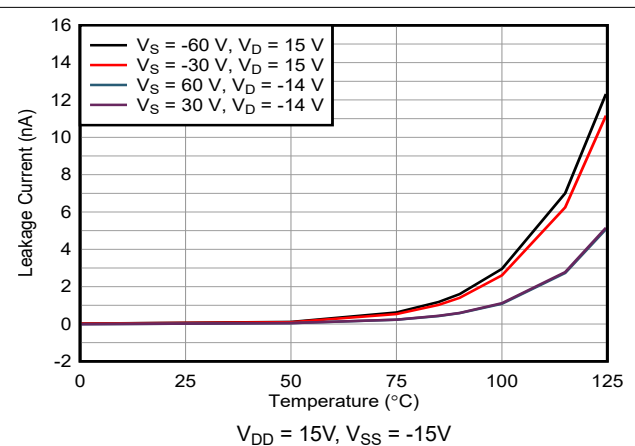
Figure 5-6. I_{D(FA)} Overvoltage Leakage Current vs Temperature
