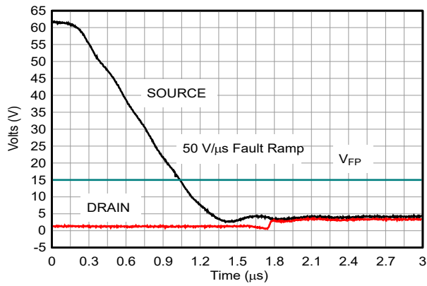
Figure 5-13. Drain Output Recovery – Positive Overvoltage
