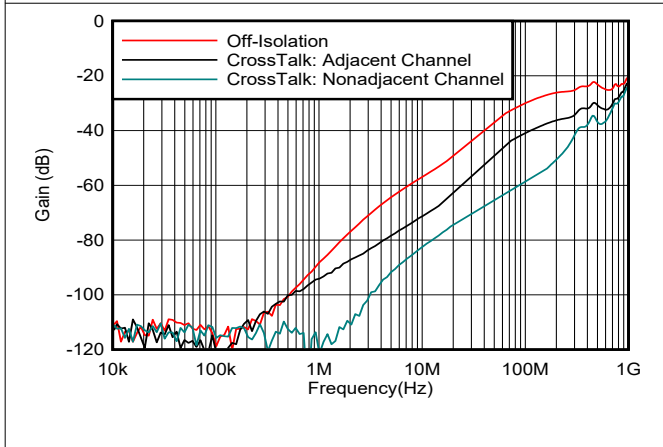
Figure 5-9. Off Isolation and Crosstalk vs Frequency
