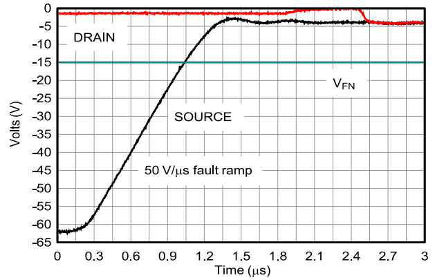
Figure 5-14. Drain Output Recovery – Negative Overvoltage
