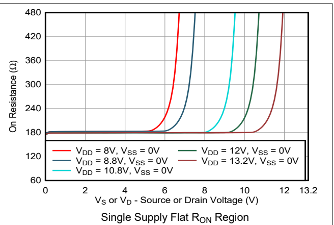
Figure 5-2. On-Resistance vs Source or Drain Voltage
