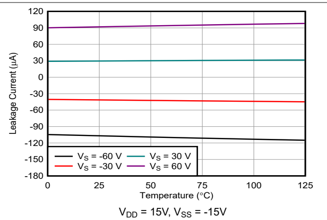
Figure 5-8. I_{S(FA)} Overvoltage Leakage Current vs Temperature
