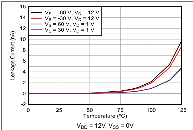
Figure 5-7. I_{D(FA)} Overvoltage Leakage Current vs Temperature
