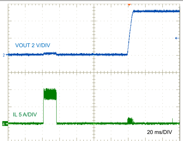
Figure 7-11. Short-Circuit Recovery
