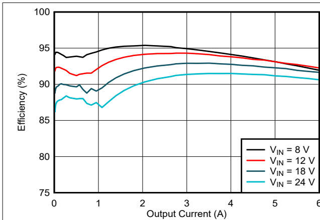
Figure 8-3. LM634x0-Q1 Efficiency
