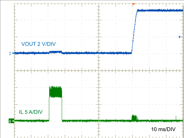
Figure 8-10. LM644x0-Q1 Short-Circuit Recovery to No Load
