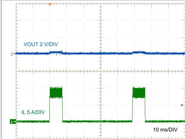
Figure 8-9. LM644x0-Q1 Short-Circuit Hiccup
