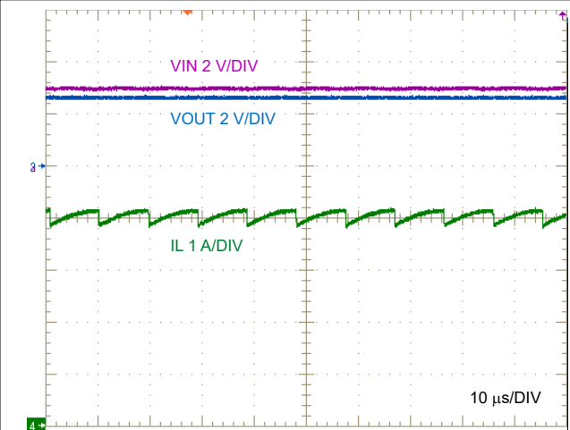
Figure 8-12. LM644x0-Q1 Frequency Foldback in Dropout, V_{IN} = 3V
