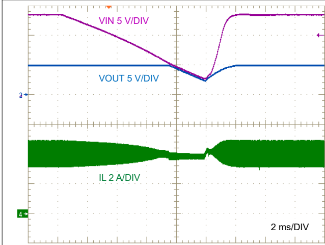
Figure 8-11. LM644x0-Q1 Line Transient and Recovery from Dropout
