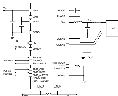
Simplified Schematic
