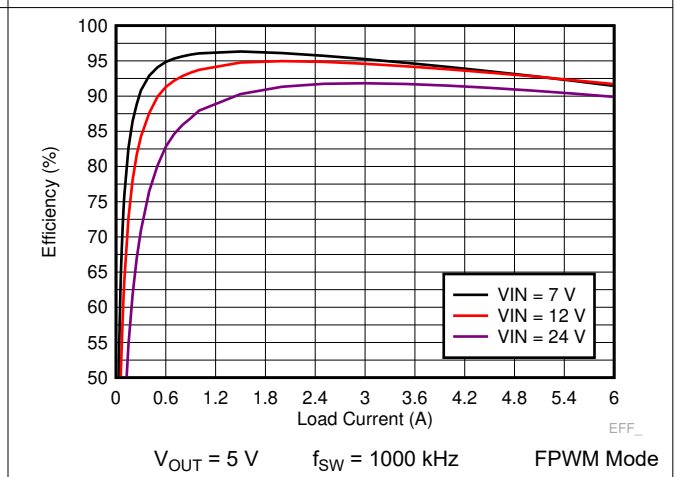
Figure 8-6. TPS7H4010-SEP Efficiency
