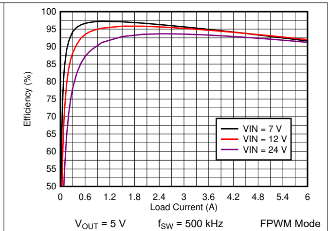
Figure 8-4. TPS7H4010-SEP Efficiency
