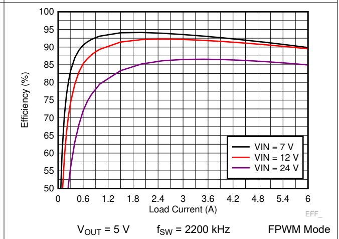
Figure 8-8. TPS7H4010-SEP Efficiency
