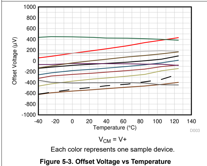
Figure 5-3. Offset Voltage vs Temperature
