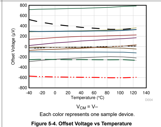
Figure 5-4. Offset Voltage vs Temperature
