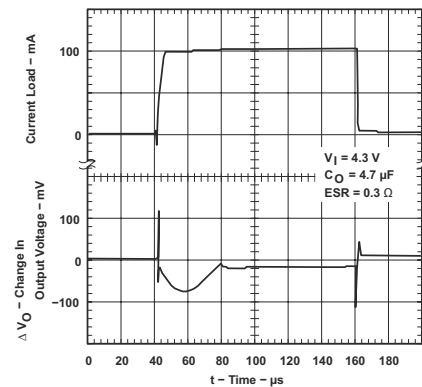
Figure 5-42. TPS76933-Q1 Load Transient Response (Legacy Chip)
