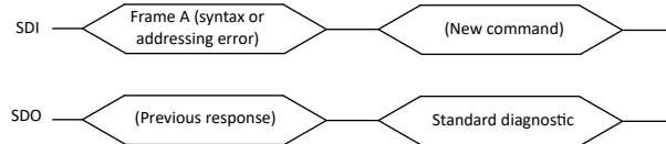
Figure 7-19. Response after a command syntax error
