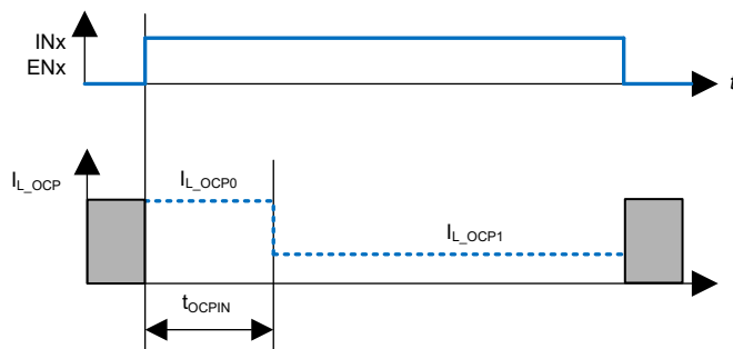
Figure 7-10. Overcurrent Threshold
