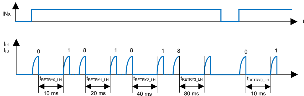
Figure 7-12. Restart Timer in Limp Home
