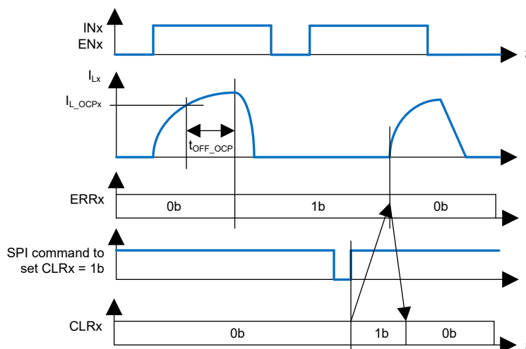
Figure 7-11. Latch OFF at Overcurrent
