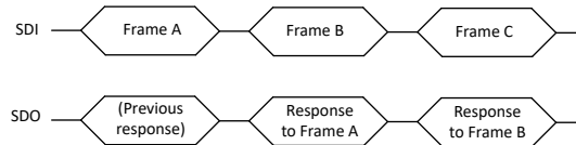
Figure 7-15. Relationship between SDI and SDO during SPI communication
