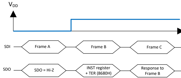
Figure 7-18. Response after coming out of Power-On reset at V DD
