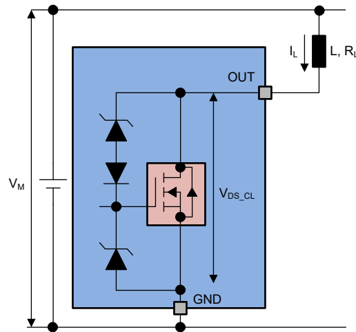
Figure 7-8. Output Clamp
