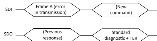
Figure 7-17. Response after a error in transmission
