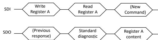
Figure 7-16. Register content sent back to microcontroller
