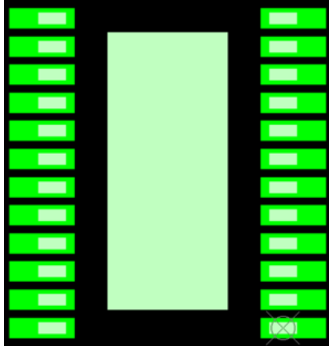
Figure 8-3. SO-24 on PWP0024T PCB Pad, White: other SO-24 leads, Green: TI PWP0024T PCB Pad
