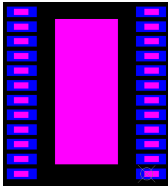
Figure 8-2. PWP0024T on another SO-24 PCB Pad, Pink: TI PWP0024T leads, Blue: other SO-24 PCB Pad
