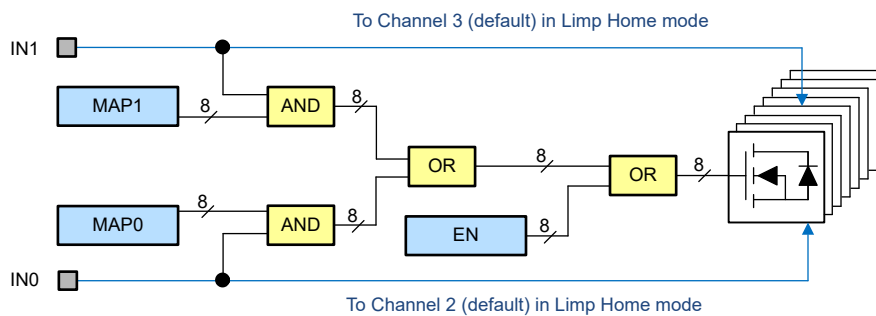
Figure 7-2. Input Mapping
