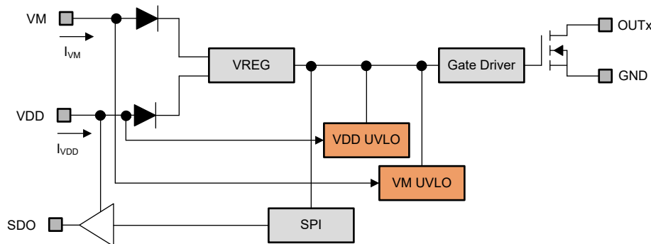
Figure 7-3. Internal Power Supply Architecture
