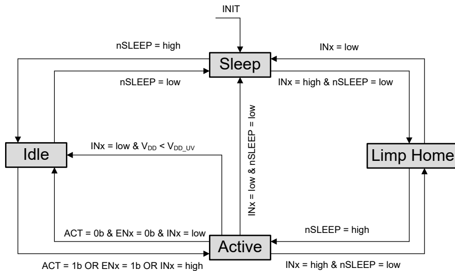
Figure 7-5. Mode of Operation State Diagram
