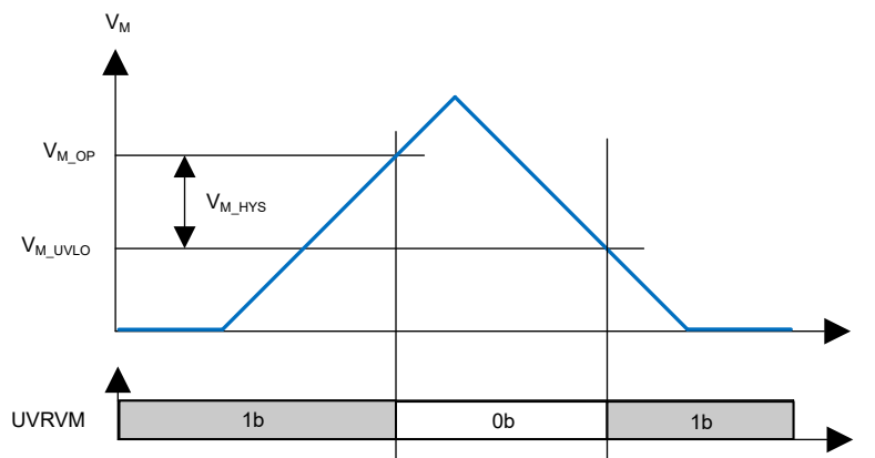
Figure 7-9. V_M Undervoltage
