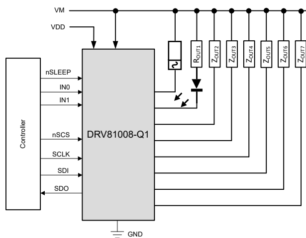
Simplified Schematic
