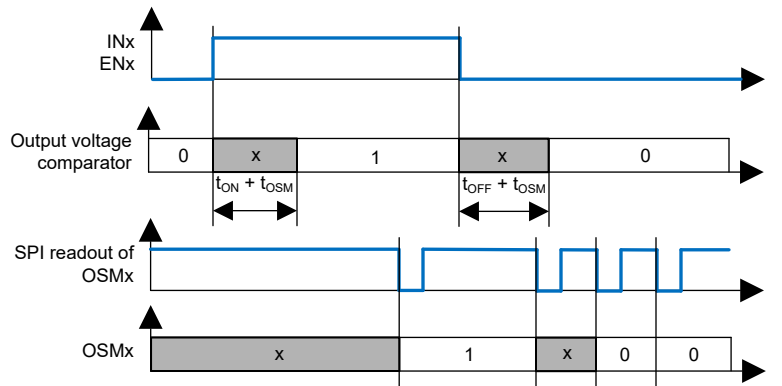
Figure 7-13. Output Status Monitor timing
