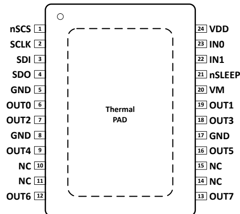
Figure 5-1. 24-Pin HTSSOP (PWP) Top View
