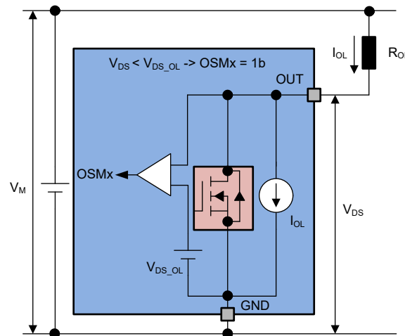
Figure 7-14. Output Status Monitor
