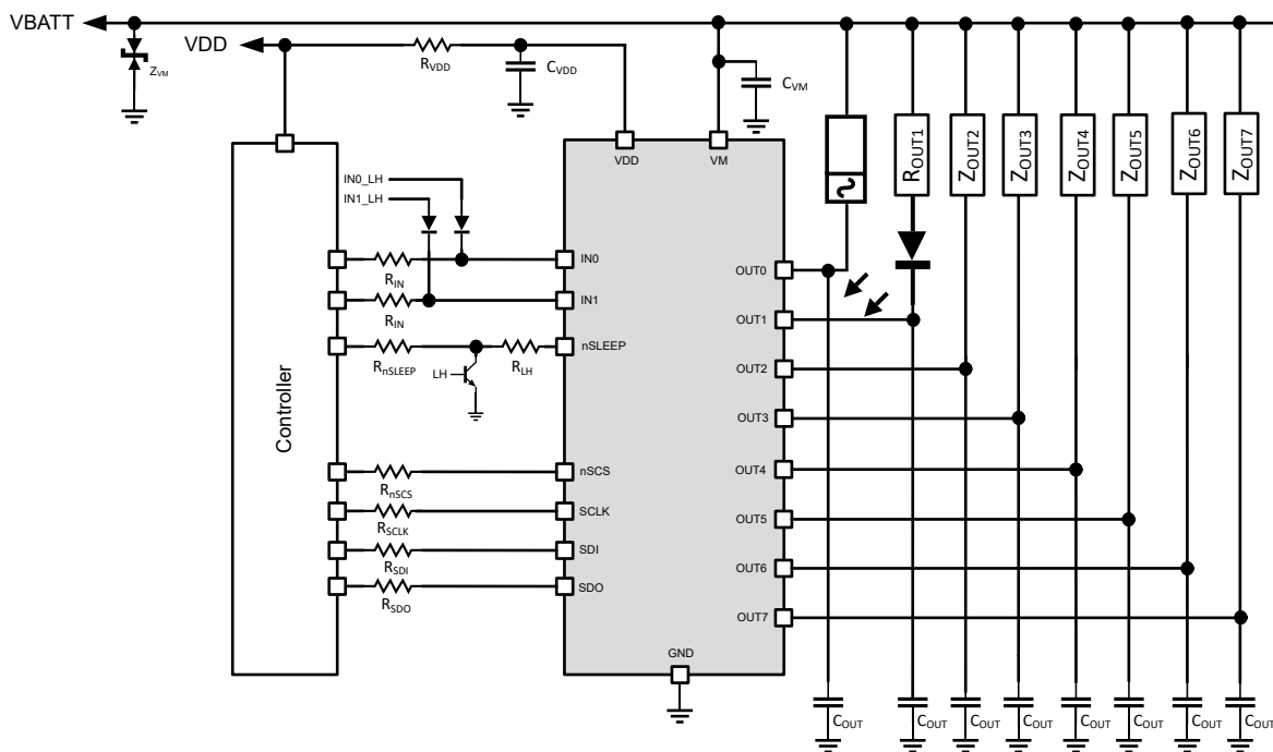
Figure 8-1. Application Schematic
